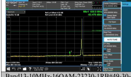
Band13-10MHz-16QAM-23230-1RB#49-30~ 1000-PASS
