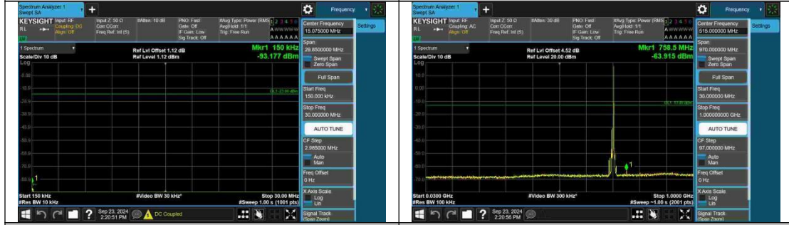
Band12-10MHz-QPSK-23095-1RB#49-0.15~30-PASS
