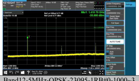
Band12-5MHz-QPSK-23095-1RB#0-1000~3 000-PASS
