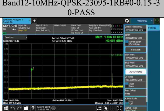
Band12-10MHz-QPSK-23095-1RB#0-1000~ 3000-PASS
