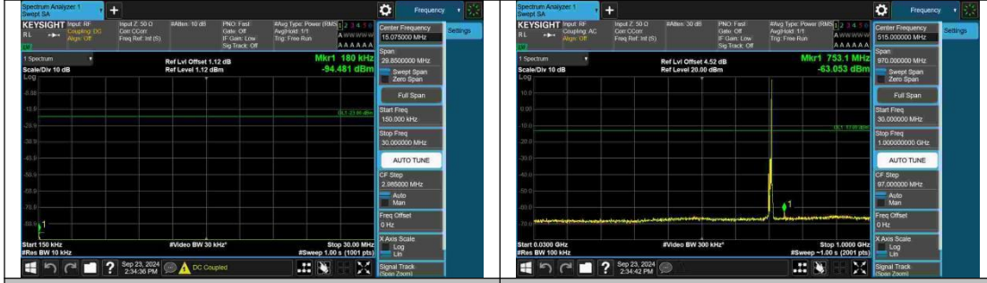
Band12-5MHz-QPSK-23155-1RB#24-0.15~30-PASS
