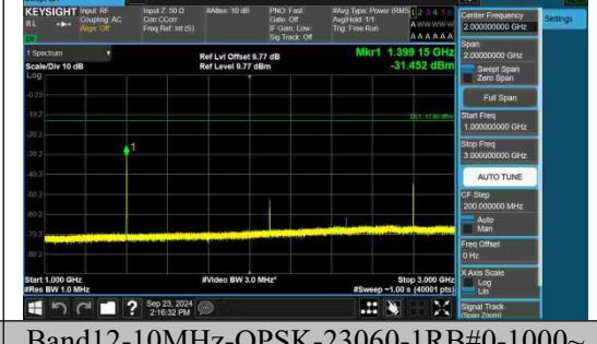
Band12-10MHz-QPSK-23060-1RB#0-1000~ 3000-PASS
