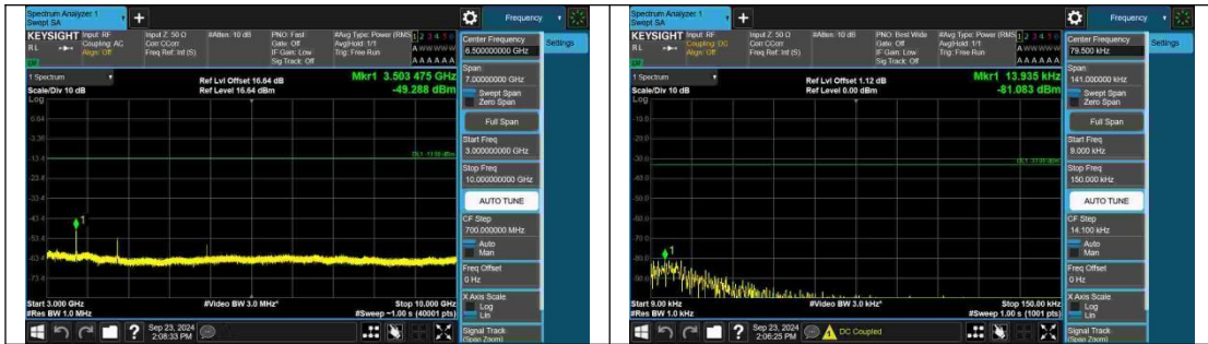
Band12-3MHz-QPSK-23025-15RB#0-3000~10000-PASS
