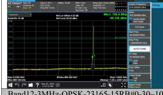
Band12-3MHz-QPSK-23165-15RB#0-30~1000-PASS
