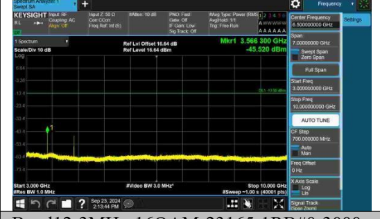
Band12-3MHz-16QAM-23165-1RB#0-3000~10000-PASS
