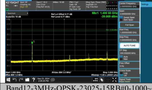
Band12-3MHz-QPSK-23025-15RB#0-1000~3000-PASS
