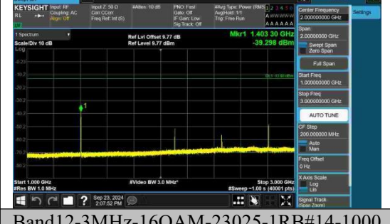
Band12-3MHz-16QAM-23025-1RB#14-1000~3000-PASS
