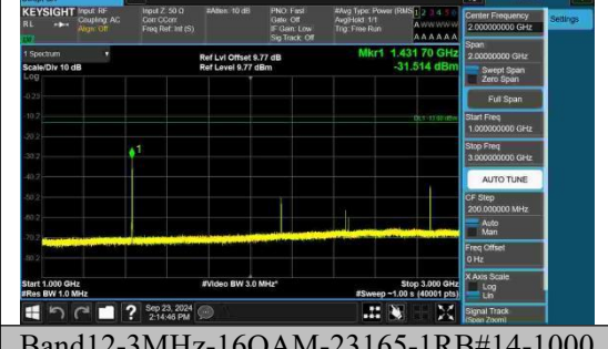
Band12-3MHz-16QAM-23165-1RB#14-1000~3000-PASS
