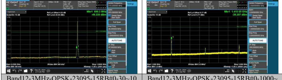
Band12-3MHz-QPSK-23095-15RB#0-30~1000-PASS
