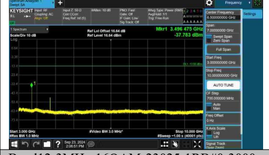
Band12-3MHz-16QAM-23025-1RB#0-3000~10000-PASS
