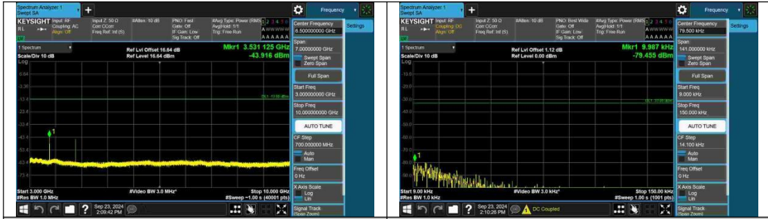
Band12-3MHz-QPSK-23095-1RB#0-3000~10000-PASS
