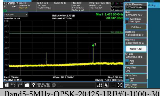
Band5-5MHz-QPSK-20425-1RB#0-1000~3000-PASS
