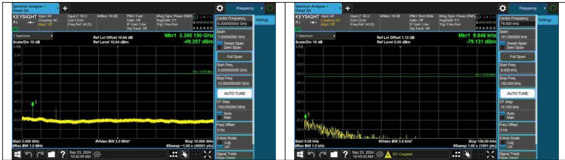
Band5-1.4MHz-16QAM-20643-1RB#5-3000 ~10000-PASS
