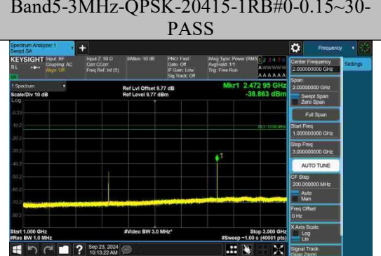
Band5-3MHz-QPSK-20415-1RB#0-1000~30 00-PASS
