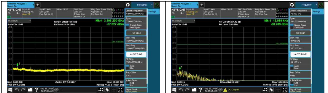
Band5-5MHz-QPSK-20425-25RB#0-3000~10000-PASS
