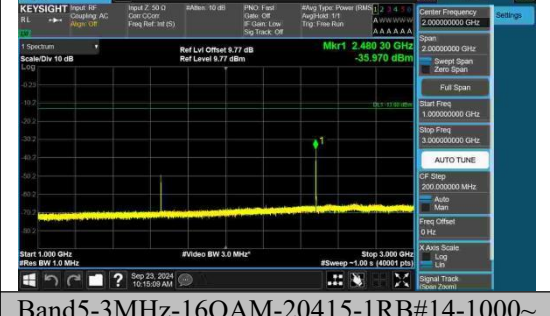
Band5-3MHz-16QAM-20415-1RB#14-1000~3000-PASS
