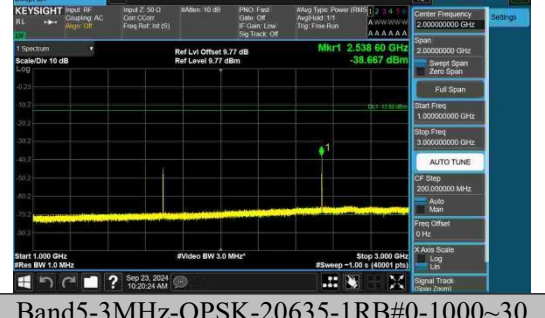
Band5-3MHz-QPSK-20635-1RB#0-1000~3000-PASS
