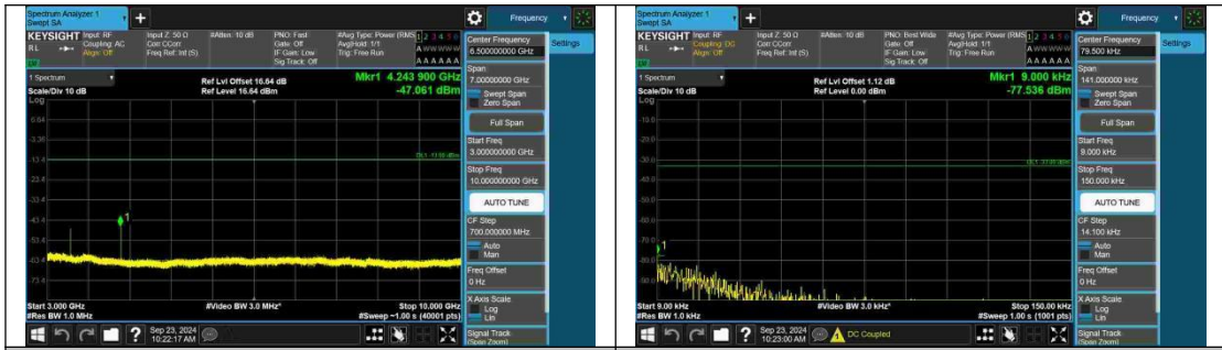
Band5-3MHz-16QAM-20635-1RB#14-3000~10000-PASS
