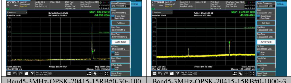
Band5-3MHz-QPSK-20415-15RB#0-30~1000-PASS
