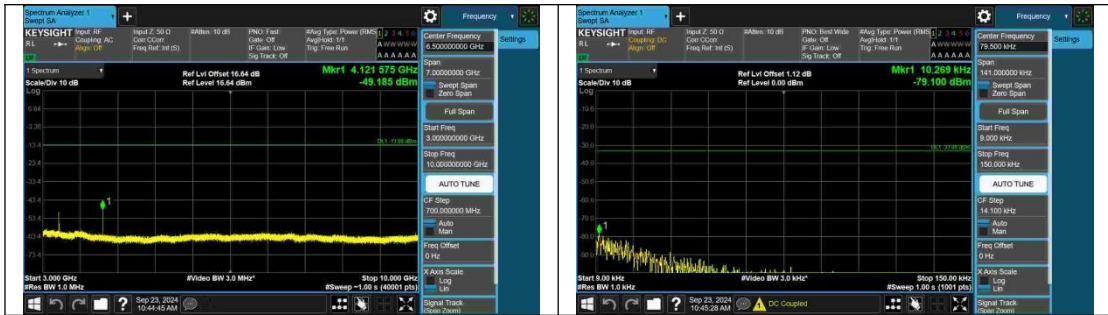
Band5-5MHz-QPSK-20425-1RB#0-3000~10000-PASS
