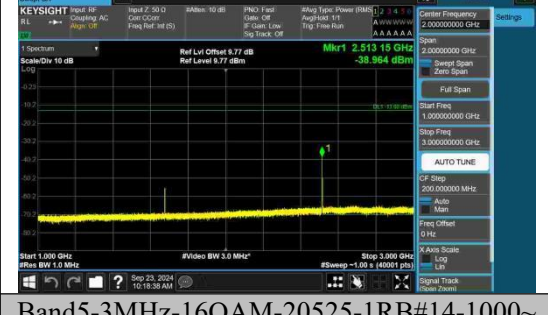
Band5-3MHz-16QAM-20525-1RB#14-1000~3000-PASS
