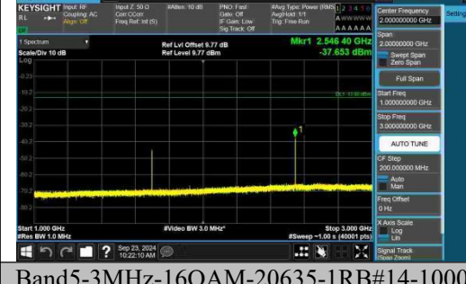
Band5-3MHz-16QAM-20635-1RB#14-1000~3000-PASS
