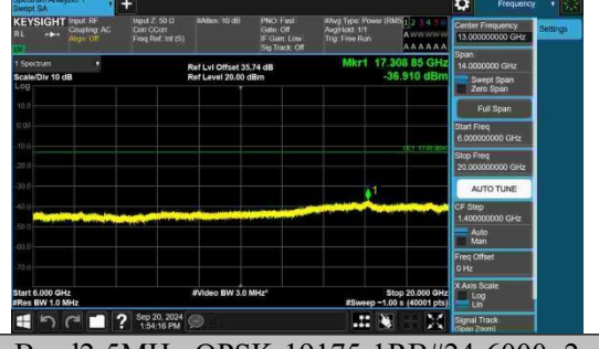
Band2-5MHz-QPSK-19175-1RB#24-6000~20000-PASS
