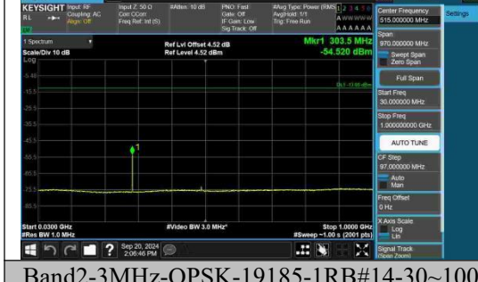
Band2-3MHz-QPSK-19185-1RB#14-30~1000-PASS
