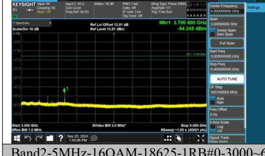
Band2-5MHz-16QAM-18625-1RB#0-3000~6 000-PASS
