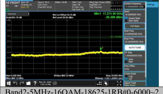
Band2-5MHz-16QAM-18625-1RB#0-6000~2 0000-PASS
