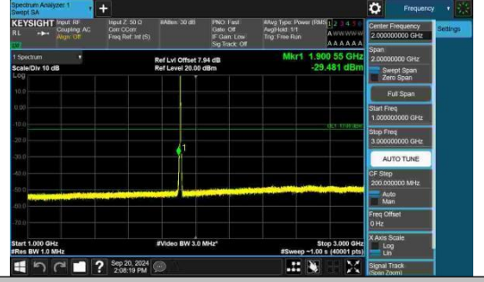
Band2-3MHz-QPSK-19185-15RB#0-1000~3000-PASS
