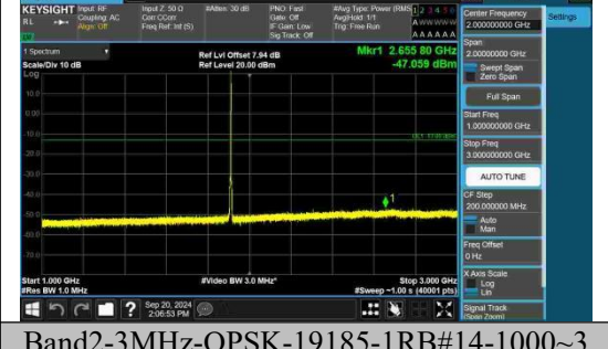
Band2-3MHz-QPSK-19185-1RB#14-1000~3000-PASS
