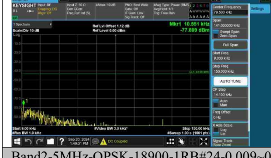
Band2-5MHz-QPSK-18900-1RB#24-0.009~0.15-PASS
