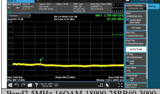
Band2-5MHz-16QAM-18900-25RB#0-3000~6000-PASS
