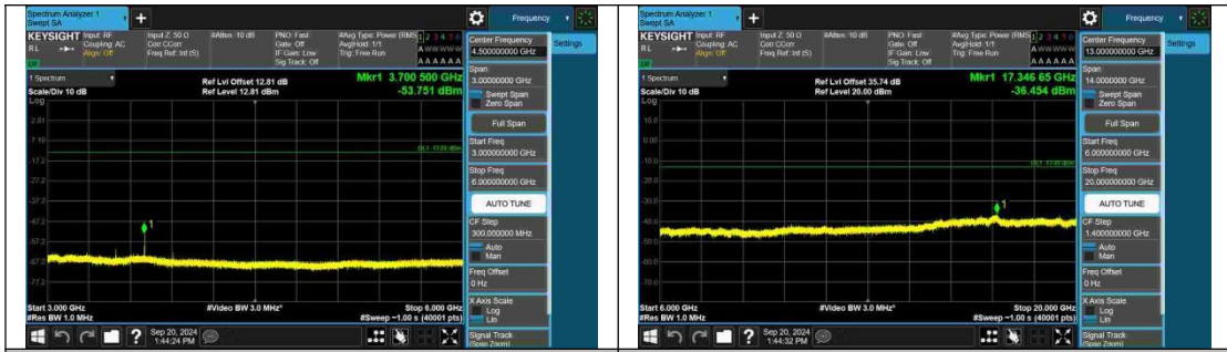
Band2-5MHz-QPSK-18625-1RB#0-3000~6000-PASS
