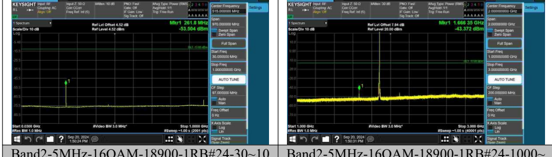
Band2-5MHz-16QAM-18900-1RB#24-30~1000-PASS
