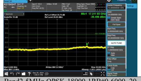
Band2-5MHz-QPSK-18900-1RB#0-6000~20000-PASS
