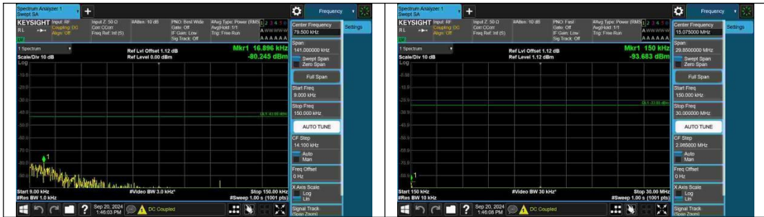
Band2-5MHz-16QAM-18625-1RB#24-0.009 ~0.15-PASS
