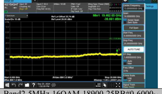
Band2-5MHz-16QAM-18900-25RB#0-6000~20000-PASS
