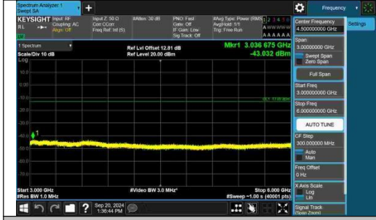
Band2-10MHz-16QAM-18900-1RB#0-3000~6000-PASS
