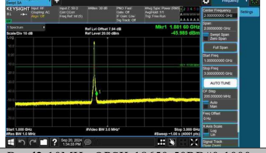
Band2-10MHz-QPSK-18650-50RB#0-1000~3000-PASS
