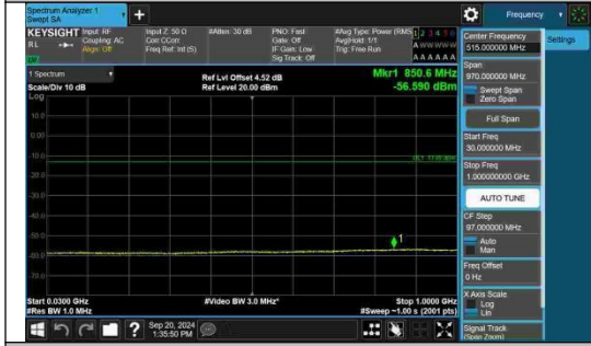
Band2-10MHz-QPSK-18900-1RB#0-30~1000-PASS
