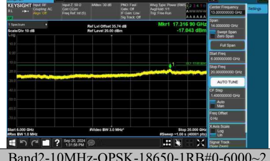
Band2-10MHz-QPSK-18650-1RB#0-6000~20000-PASS
