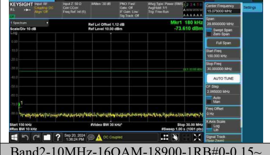
Band2-10MHz-16QAM-18900-1RB#0-0.15~30-PASS
