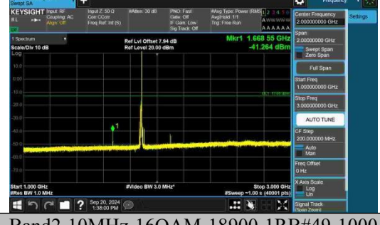
Band2-10MHz-16QAM-18900-1RB#49-1000~3000-PASS
