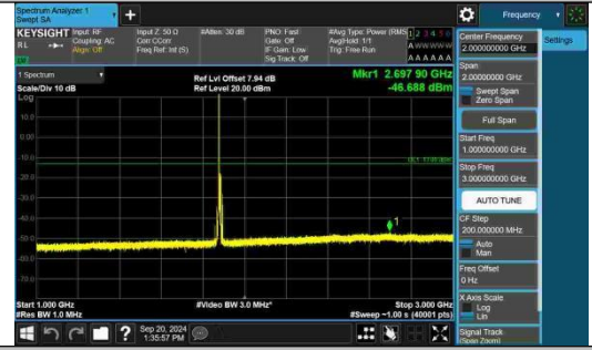
Band2-10MHz-QPSK-18900-1RB#0-1000~3000-PASS
