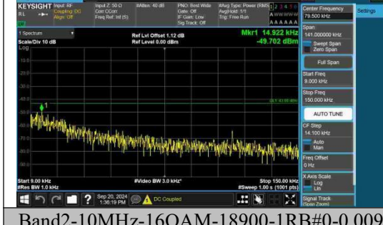
Band2-10MHz-16QAM-18900-1RB#0-0.009~0.15-PASS
