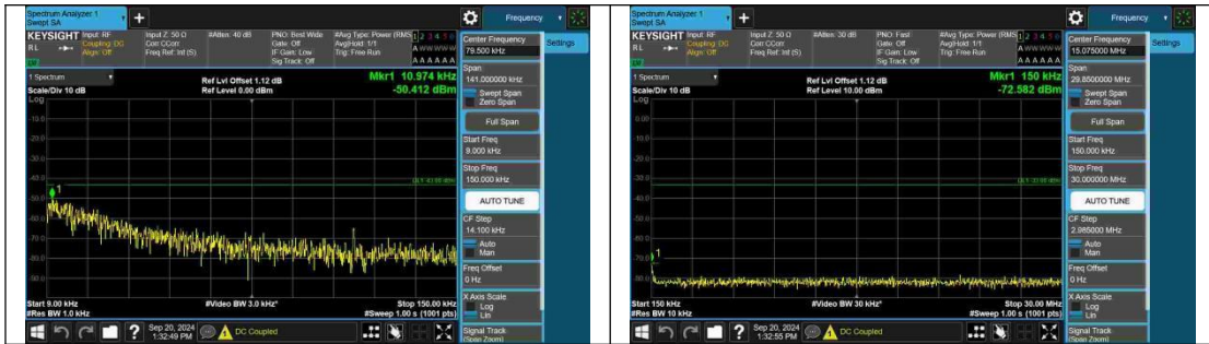
Band2-10MHz-QPSK-18650-1RB#49-0.009~0.15-PASS
