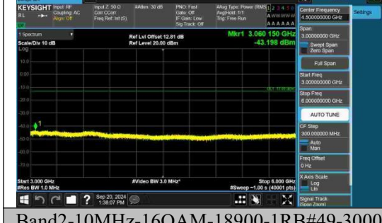
Band2-10MHz-16QAM-18900-1RB#49-3000~6000-PASS
