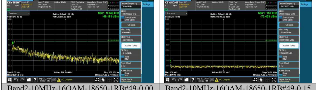
Band2-10MHz-16QAM-18650-1RB#49-0.009~0.15-PASS
