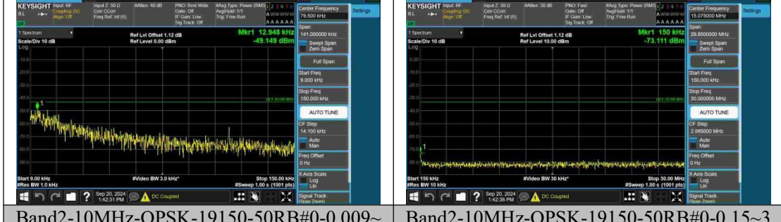
Band2-10MHz-QPSK-19150-50RB#0-0.009~0.15-PASS
