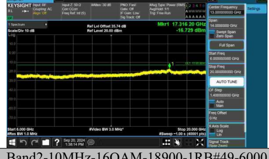
Band2-10MHz-16QAM-18900-1RB#49-6000~20000-PASS
