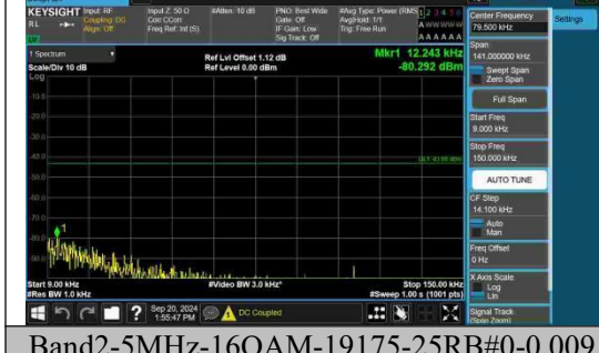
Band2-5MHz-16QAM-19175-25RB#0-0.009~0.15-PASS
