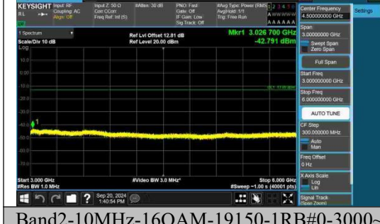
Band2-10MHz-16QAM-19150-1RB#0-3000~6000-PASS
