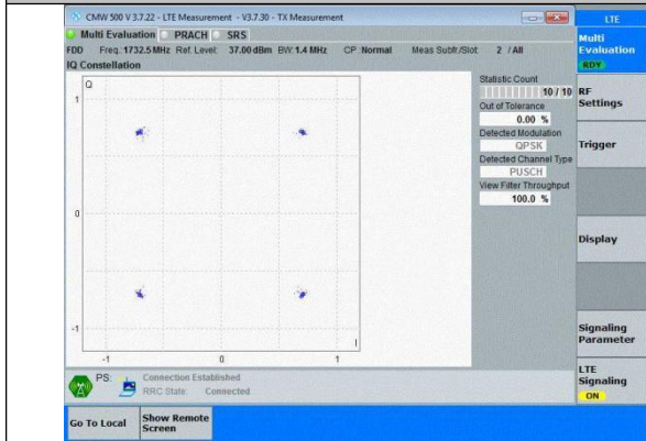
Band4-1.4MHz-QPSK-20175-6RB#0-PASS
