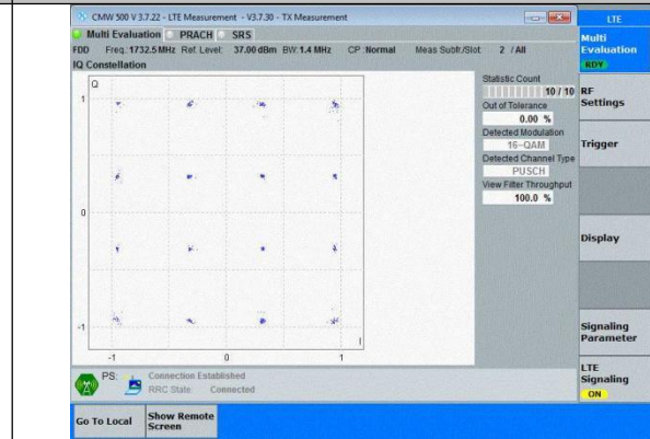
Band4-1.4MHz-16QAM-20175-6RB#0-PASS
