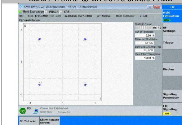
Band4-1.4MHz-QPSK-20393-6RB#0-PASS
