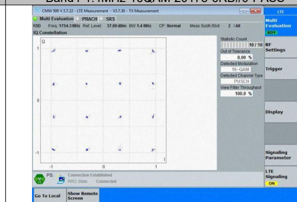
Band4-1.4MHz-16QAM-20393-6RB#0-PASS
