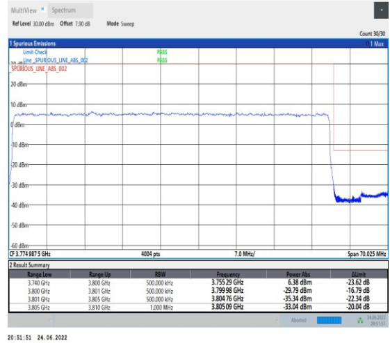
1-N78-3700-3800-PC2-30-60-H-3-DFT-PI2BPSK-Outer_Full-162@0-Ant1-PASS-see graph
