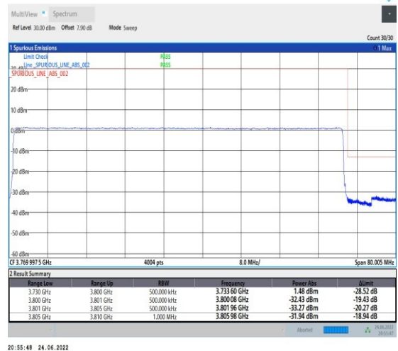
1-N78-3700-3800-PC2-30-70-H-6-CP-QPSK-Outer_Full-189@0-Ant1-PASS-see graph
