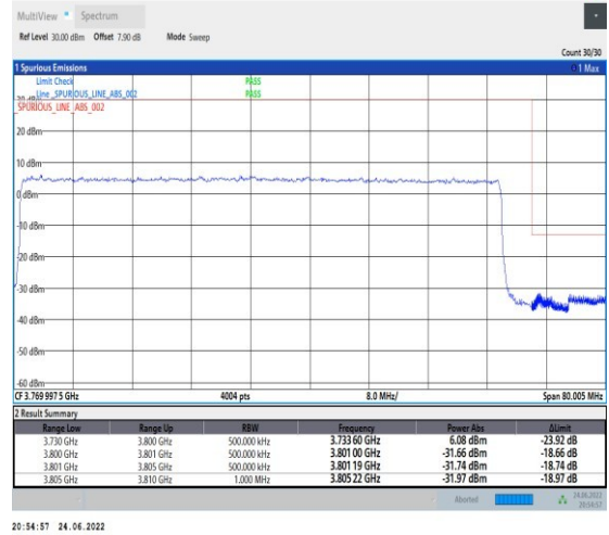
1-N78-3700-3800-PC2-30-70-H-3-DFT-PI2BPSK-Outer_Full-180@0-Ant1-PASS-see graph
