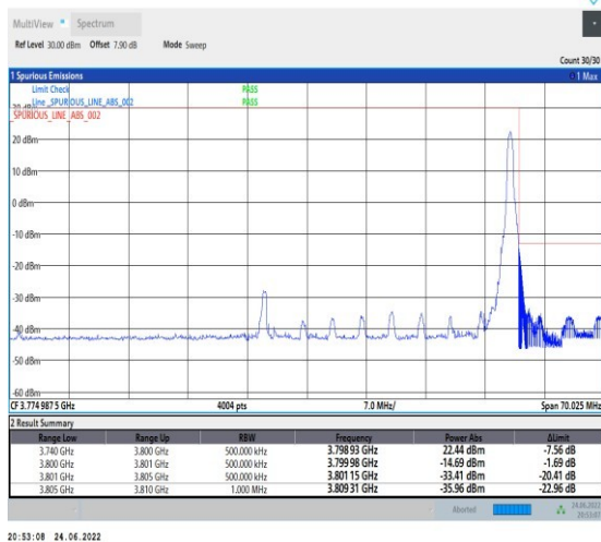
1-N78-3700-3800-PC2-30-60-H-5-CP-QPSK-Edge_1RB_Right-1@161-Ant1-PASS-see graph
