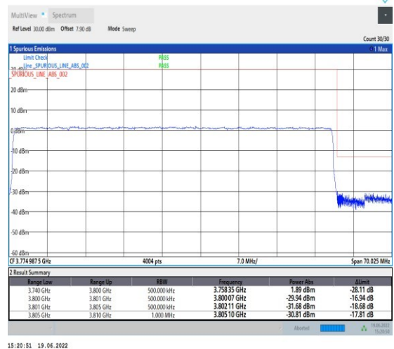
1-N78-3700-3800-PC2-30-60-H-6-CP-QPSK-Outer_Full-162@0-Ant1-PASS-see graph
