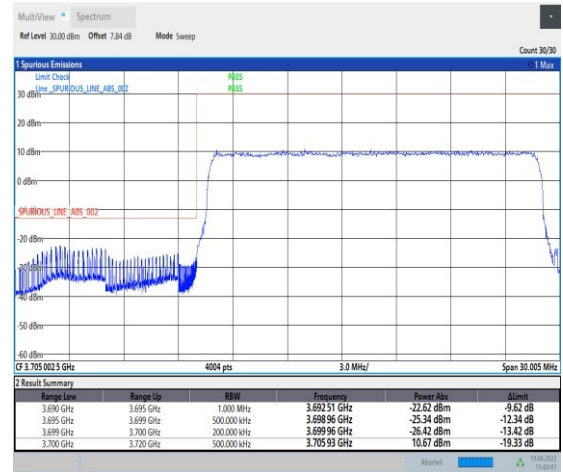
1-N78-3700-3800-PC2-30-20-L-3-DFT-PI2BPSK-Outer_Full-50@0-Ant1-PASS-see graph
