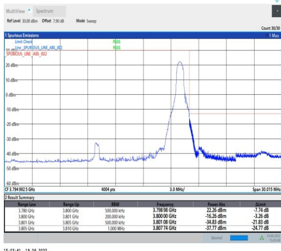
1-N78-3700-3800-PC2-30-20-H-2-DFT-PI2BPSK-Edge_1RB_Right-1@50-Ant1-PASS-see graph
