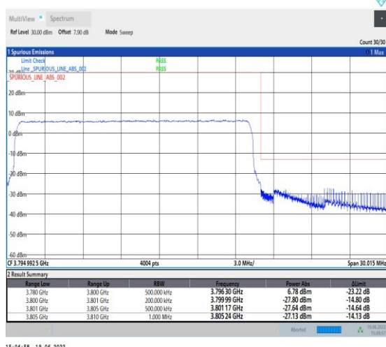
1-N78-3700-3800-PC2-30-20-H-6-CP-QPSK-Outer_Full-51@0-Ant1-PASS-see graph
