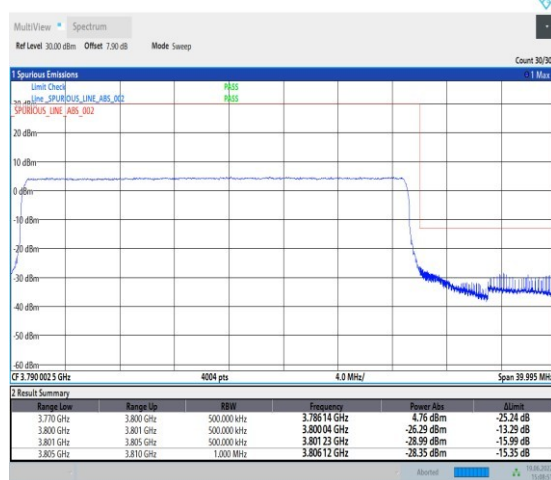
1-N78-3700-3800-PC2-30-30-H-6-CP-QPSK-Outer_Full-78@0-Ant1-PASS-see graph
