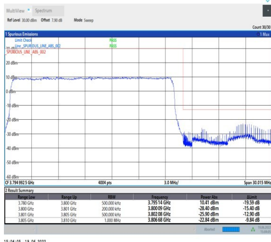
1-N78-3700-3800-PC2-30-20-H-3-DFT-PI2BPSK-Outer_Full-50@0-Ant1-PASS-see graph
