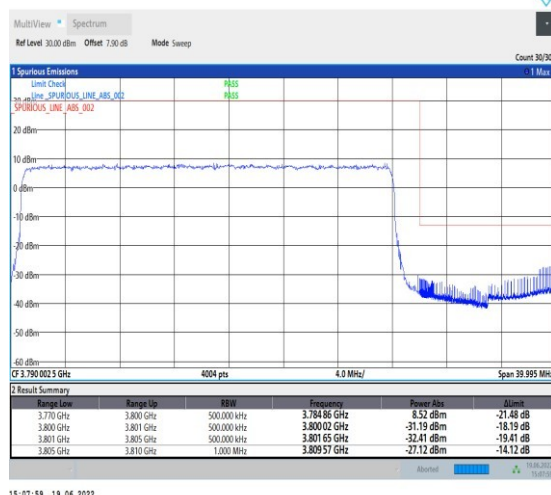
1-N78-3700-3800-PC2-30-30-H-3-DFT-PI2BPSK-Outer_Full-75@0-Ant1-PASS-see graph
