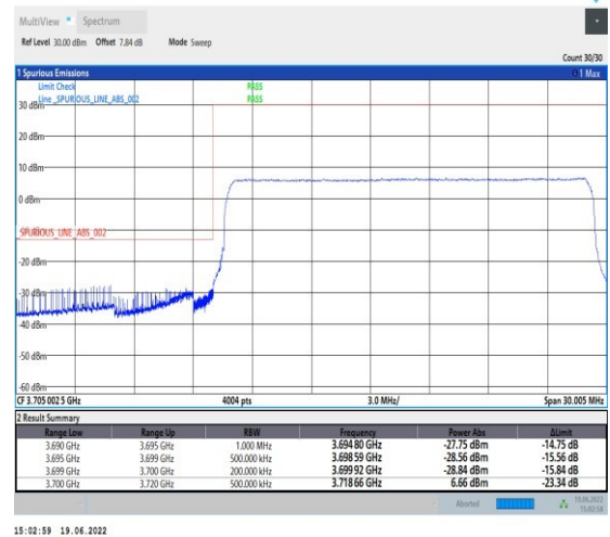
1-N78-3700-3800-PC2-30-20-L-6-CP-QPSK-Outer_Full-51@0-Ant1-PASS-see graph
