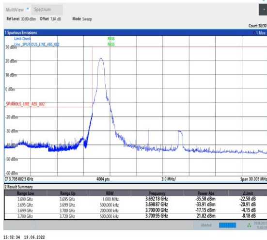
1-N78-3700-3800-PC2-30-20-L-4-CP-QPSK-Edge_1RB_Left-1@0-Ant1-PASS-see graph
