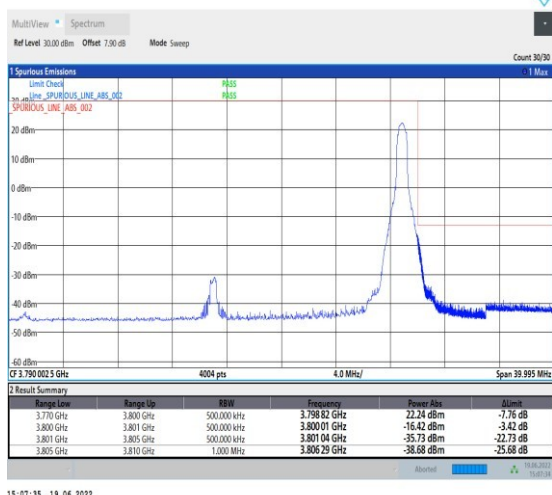
1-N78-3700-3800-PC2-30-30-H-2-DFT-PI2BPSK-Edge_1RB_Right-1@77-Ant1-PASS-see graph
