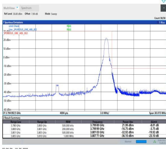
1-N78-3700-3800-PC2-30-20-H-5-CP-QPSK-Edge_1RB_Right-1@50-Ant1-PASS-see graph
