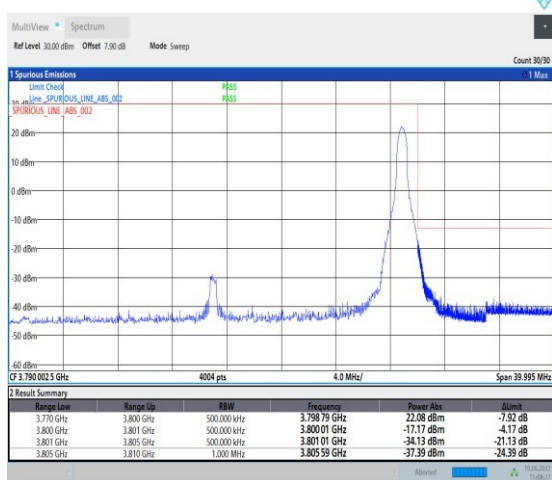
1-N78-3700-3800-PC2-30-30-H-5-CP-QPSK-Edge_1RB_Right-1@77-Ant1-PASS-see graph
