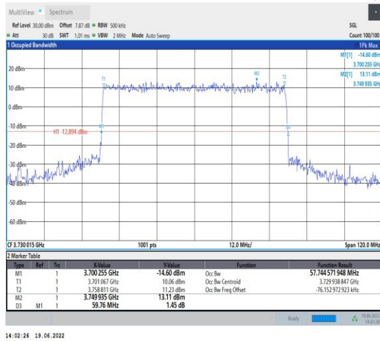
1-N78-3700-3800-PC2-30-60-L-1-DFT-QPSK-Outer_Full-162@0-Ant1-57.745-59.760-≤60-PASS
