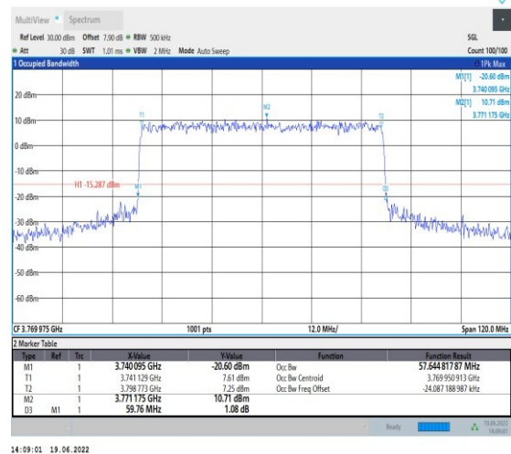
1-N78-3700-3800-PC2-30-60-H-6-CP-QPSK-Outer_Full-162@0-Ant1-57.645-59.760-≤60-PASS
