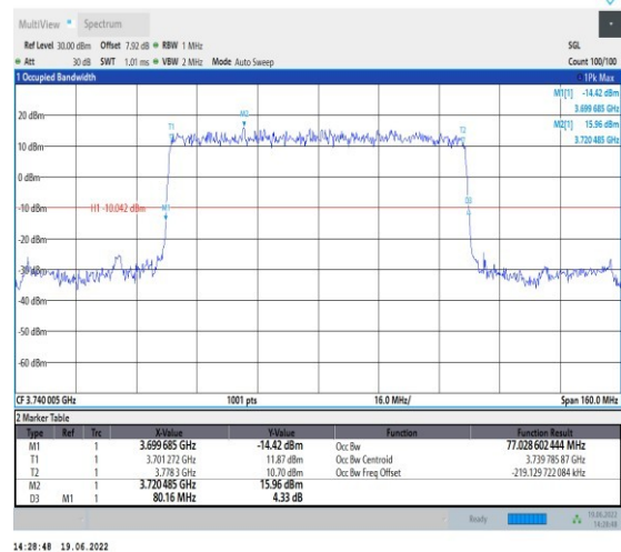
1-N78-3700-3800-PC2-30-80-L-2-DFT-PI2BPSK-Outer _Full-216@0-Ant1-77.029-80.160-≤80-PASS
