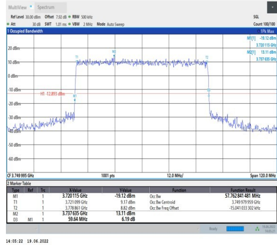
1-N78-3700-3800-PC2-30-60-M-1-DFT-QPSK-Outer_Full-162@0-Ant1-57.763-59.640-≤60-PASS
