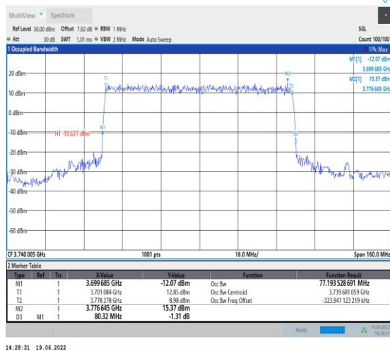
1-N78-3700-3800-PC2-30-80-L-1-DFT-QPSK-Outer _Full-216@0-Ant1-77.194-80.320-≤80-PASS
