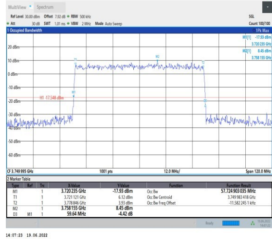
1-N78-3700-3800-PC2-30-60-M-9-CP-256QAM-Outer_Full-162@0-Ant1-57.725-59.640-≤60-PASS
