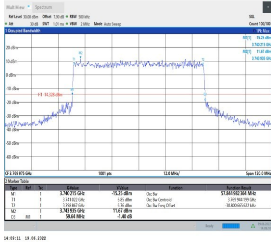
1-N78-3700-3800-PC2-30-60-H-7-CP-16QAM-Outer _Full-162@0-Ant1-57.845-59.640-≤60-PASS
