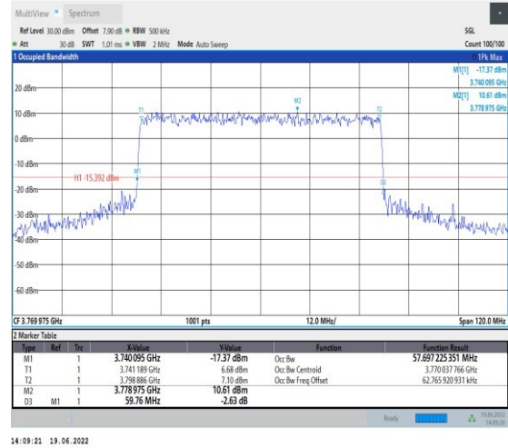
1-N78-3700-3800-PC2-30-60-H-8-CP-64QAM-Outer _Full-162@0-Ant1-57.697-59.760-≤60-PASS
