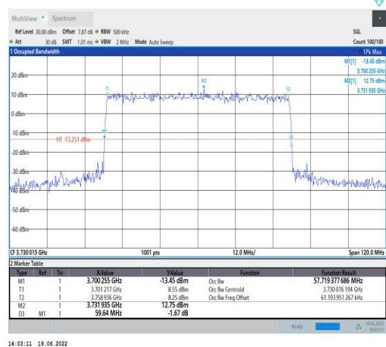
1-N78-3700-3800-PC2-30-60-L-4-DFT-64QAM-Outer_Full-162@0-Ant1-57.719-59.640-≤60-PASS
