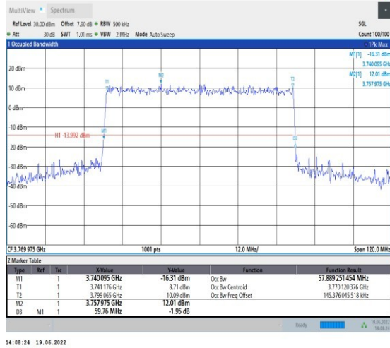
1-N78-3700-3800-PC2-30-60-H-3-DFT-16QAM-Outer_Full-162@0-Ant1-57.889-59.760-≤60-PASS
