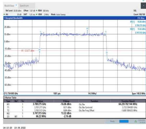
1-N78-3700-3800-PC2-30-70-L-1-DFT-QPSK-Outer _Full-180@0-Ant1-64.236-66.220-≤70-PASS
