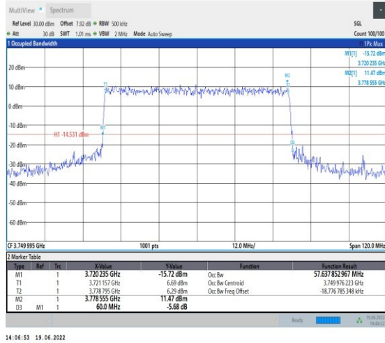
1-N78-3700-3800-PC2-30-60-M-8-CP-64QAM-Outer_Full-162@0-Ant1-57.638-60.000-≤60-PASS
