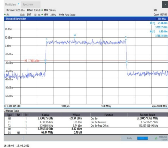
1-N78-3700-3800-PC2-30-70-H-9-CP-256QAM-Outer _Full-189@0-Ant1-67.601-69.440-≤70-PASS
