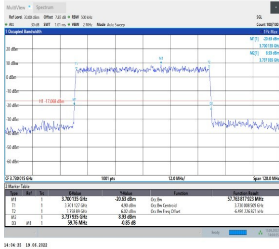
1-N78-3700-3800-PC2-30-60-L-9-CP-256QAM-Outer_Full-162@0-Ant1-57.764-59.760-≤60-PASS
