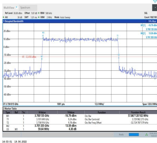
1-N78-3700-3800-PC2-30-60-L-3-DFT-16QAM-Outer_Full-162@0-Ant1-57.867-59.640-≤60-PASS
