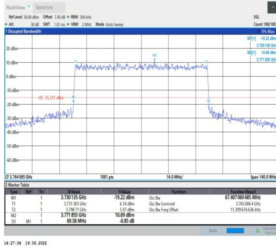
1-N78-3700-3800-PC2-30-70-H-8-CP-64QAM-Outer _Full-189@0-Ant1-67.407-69.580-≤70-PASS
