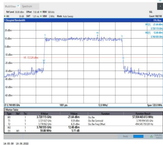
1-N78-3700-3800-PC2-30-60-M-3-DFT-16QAM-Outer_Full-162@0-Ant1-57.934-59.880-≤60-PASS
