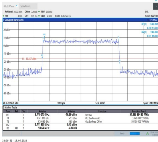
1-N78-3700-3800-PC2-30-60-H-9-CP-256QAM-Outer _Full-162@0-Ant1-57.834-59.640-≤60-PASS
