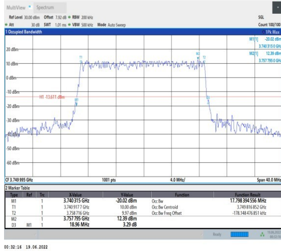
1-N78-3700-3800-PC2-30-20-M-4-DFT-64QAM-Out er_Full-50@0-Ant1-17.798-18.960-≤20-PASS
