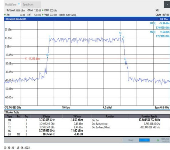
1-N78-3700-3800-PC2-30-20-M-5-DFT-256QAM-Out er_Full-50@0-Ant1-17.805-18.760-≤20-PASS
