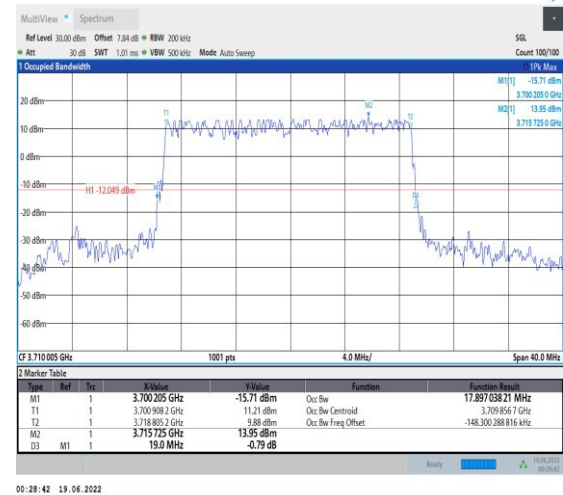
1-N78-3700-3800-PC2-30-20-L-2-DFT-PI2BPSK-Outer_Full-50@0-Ant1-17.897-19.000-≤20-PASS
