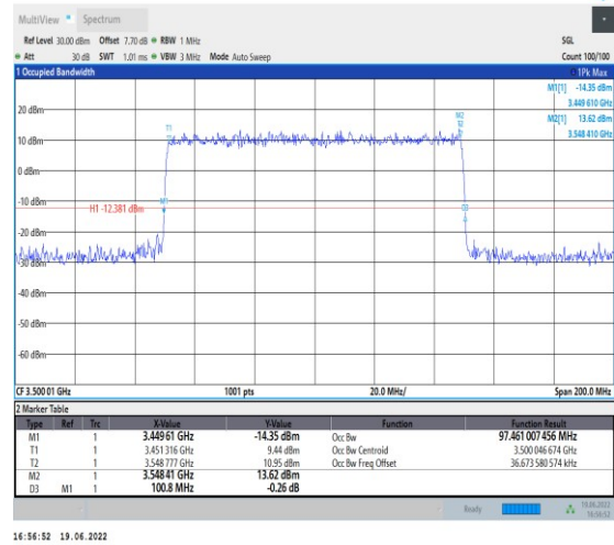
1-N78-3450-3550-PC2-30-100-L-7-CP-16QAM-Outer_Full-273@0-Ant1-97.461-100.800-≤100-PASS
