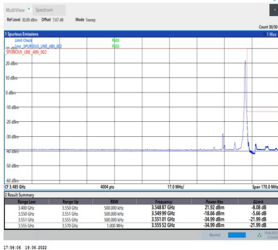
1-N78-3450-3550-PC2-30-30-H-5-CP-QPSK-Edge_1RB_Right-1@77-Ant1-PASS-see graph
