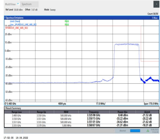
1-N78-3450-3550-PC2-30-30-H-3-DFT-PI2BPSK-Outer_Full-75@0-Ant1-PASS-see graph
