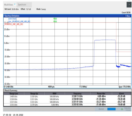
1-N78-3450-3550-PC2-30-30-H-6-CP-QPSK-Outer_Full-78@0-Ant1-PASS-see graph
