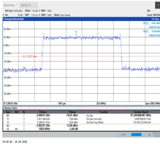
1-N78-3450-3550-PC2-30-100-L-6-CP-QPSK-Outer_Full-273@0-Ant1-97.245-100.800-≤100-PASS
