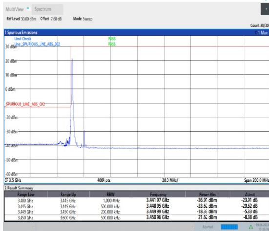
1-N78-3450-3550-PC2-30-20-L-4-CP-QPSK-Edge_1RB_Left-1@0-Ant1-PASS-see graph
