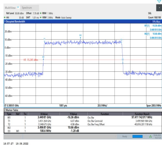
1-N78-3450-3550-PC2-30-100-L-9-CP-256QAM-Outer_Full-273@0-Ant1-97.411-100.600-≤100-PASS
