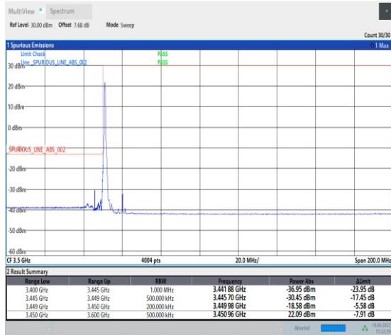
1-N78-3450-3550-PC2-30-20-L-1-DFT-PI2BPSK-Edge_1RB_Left-1@0-Ant1-PASS-see graph
