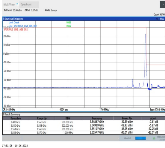
1-N78-3450-3550-PC2-30-30-H-2-DFT-PI2BPSK-Edge_1RB_Right-1@77-Ant1-PASS-see graph
