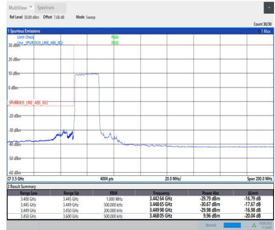
1-N78-3450-3550-PC2-30-20-L-3-DFT-PI2BPSK-Outer_Full-50@0-Ant1-PASS-see graph
