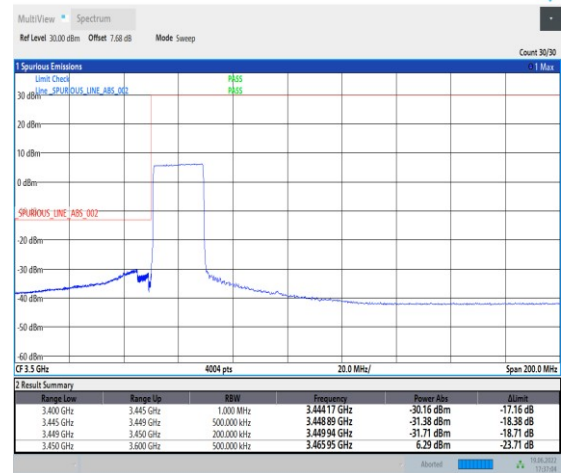
1-N78-3450-3550-PC2-30-20-L-6-CP-QPSK-Outer_Full-51@0-Ant1-PASS-see graph
