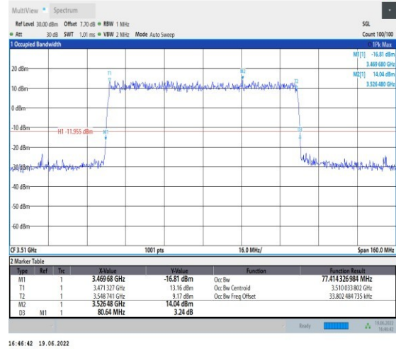
1-N78-3450-3550-PC2-30-80-H-7-CP-16QAM-Outer_Full-217@0-Ant1-77.414-80.640-≤80-PASS
