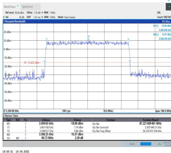
1-N78-3450-3550-PC2-30-90-H-9-CP-256QAM-Outer _Full-245@0-Ant1-87.222-90.720-≤90-PASS
