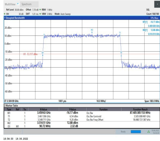
1-N78-3450-3550-PC2-30-90-H-8-CP-64QAM-Outer _Full-245@0-Ant1-87.405-90.720-≤90-PASS
