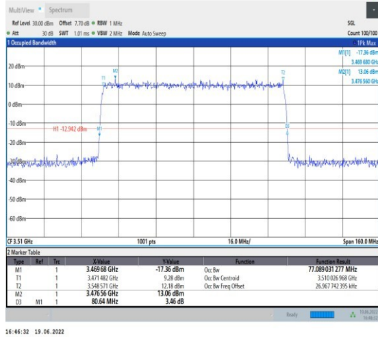
1-N78-3450-3550-PC2-30-80-H-6-CP-QPSK-Outer_Full-217@0-Ant1-77.089-80.640-≤80-PASS
