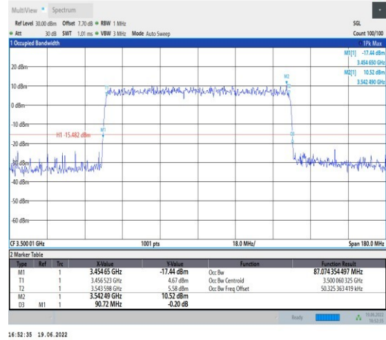
1-N78-3450-3550-PC2-30-90-M-9-CP-256QAM-Outer_Full-245@0-Ant1-87.074-90.720-≤90-PASS
