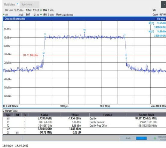
1-N78-3450-3550-PC2-30-90-H-7-CP-16QAM-Outer _Full-245@0-Ant1-87.311-90.720-≤90-PASS
