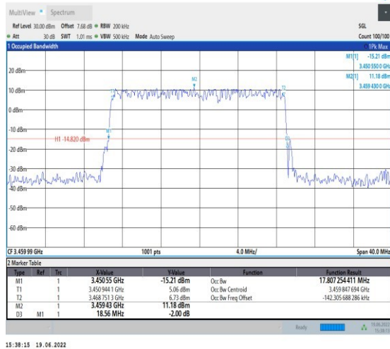
1-N78-3450-3550-PC2-30-20-L-5-DFT-256QAM-Out er_Full-50@0-Ant1-17.807-18.560-≤20-PASS
