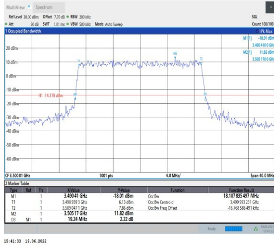
1-N78-3450-3550-PC2-30-20-M-8-CP-64QAM-Outer _Full-51@0-Ant1-18.108-19.240-≤20-PASS
