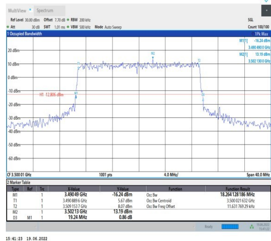
1-N78-3450-3550-PC2-30-20-M-7-CP-16QAM-Outer_Full-51@0-Ant1-18.264-19.240-≤20-PASS
