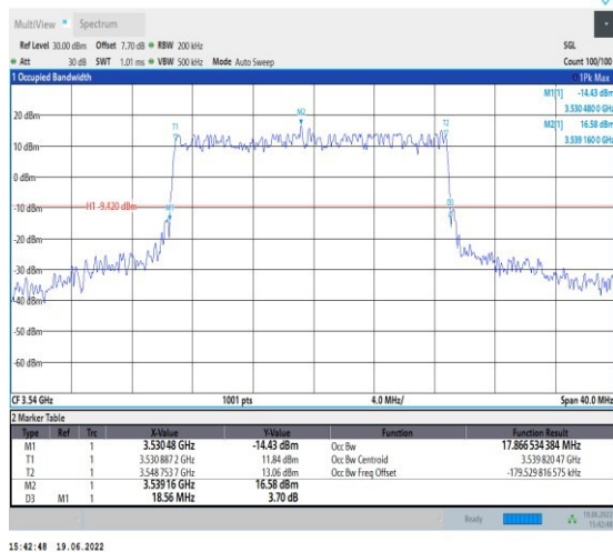
1-N78-3450-3550-PC2-30-20-H-1-DFT-QPSK-Outer _Full-50@0-Ant1-17.867-18.560-≤20-PASS
