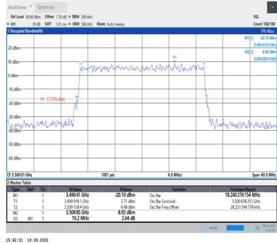
1-N78-3450-3550-PC2-30-20-M-9-CP-256QAM-Outer _Full-51@0-Ant1-18.24-19.200-≤20-PASS
