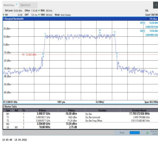
1-N78-3450-3550-PC2-30-20-M-4-DFT-64QAM-Out er_Full-50@0-Ant1-17.796-18.880-≤20-PASS
