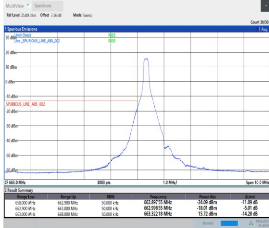
1-N71--15-5-L-1-DFT-PI2BPSK-Edge_1RB_Left-1@0-Ant1-PASS-see graph
