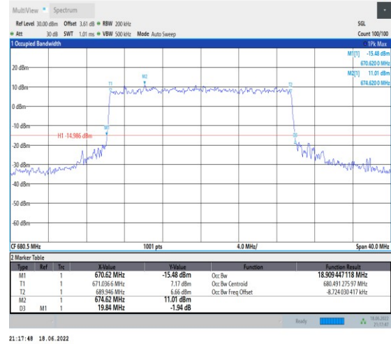
1-N71--15-20-M-8-CP-64QAM-Outer_Full-106@0-A nt1-18.909-19.840-≤20-PASS
