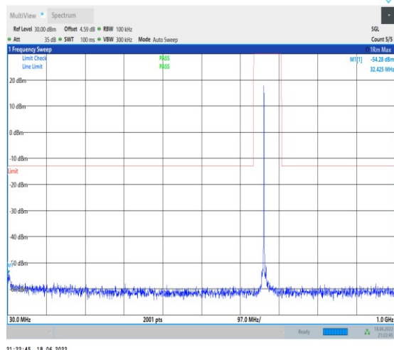
1-N71--15-20-M-1-DFT-PI2BPSK-Inner_1RB_Left-1 @1-30-1000-Ant1--54.28--13-PASS
