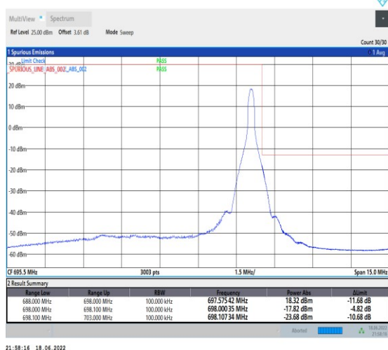
1-N71--15-10-H-5-CP-QPSK-Edge_1RB_Right-1@51- Ant1-PASS-see graph
