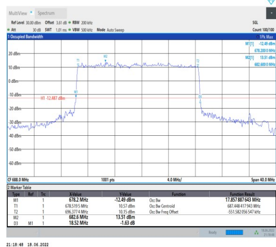
1-N71--15-20-H-1-DFT-QPSK-Outer_Full-100@0-An t1-17.858-18.520-≤20-PASS
