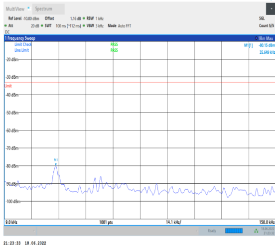
1-N71--15-20-H-1-DFT-PI2BPSK-Inner_1RB_Left-1 @1-0.009-0.15-Ant1--80.15--33-PASS
