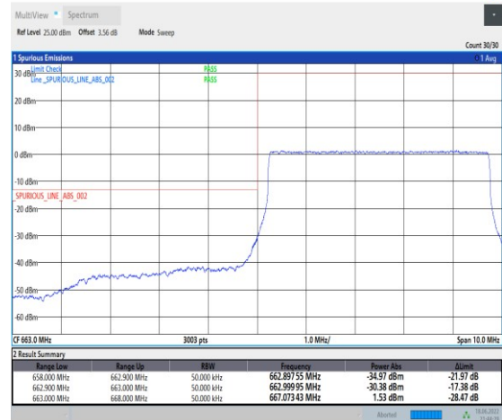
1-N71--15-5-L-6-CP-QPSK-Outer_Full-25@0-Ant1-PASS-see graph
