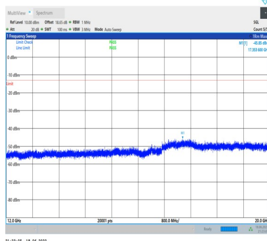
1-N71--15-20-M-1-DFT-PI2BPSK-Inner_1RB_Left-1 @1-12000-20000-Ant1--45.85--13-PASS
