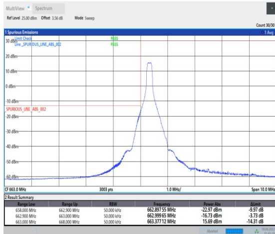
1-N71--15-5-L-4-CP-QPSK-Edge_1RB_Left-1@0-Ant1-PASS-see graph
