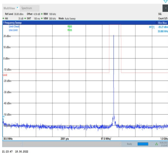
1-N71--15-20-H-1-DFT-PI2BPSK-Inner_1RB_Left-1 @1-30-1000-Ant1--55.27--13-PASS
