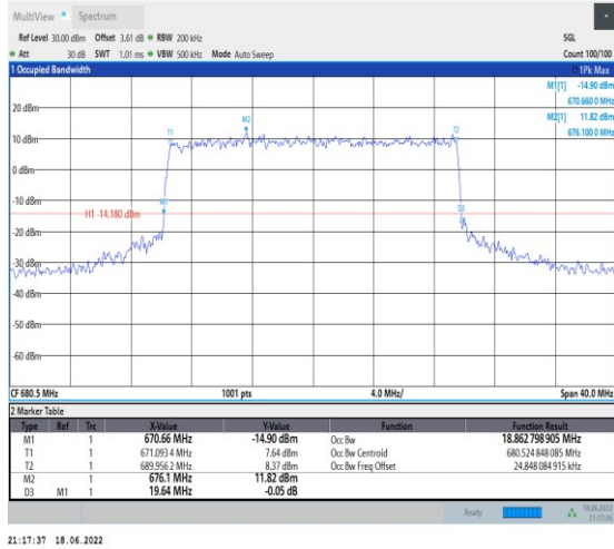
1-N71--15-20-M-7-CP-16QAM-Outer_Full-106@0-An t1-18.863-19.640-≤20-PASS
