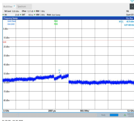
1-N71--15-20-M-1-DFT-PI2BPSK-Inner_1RB_Left-1 @1-3000-12000-Ant1--49.74--13-PASS
