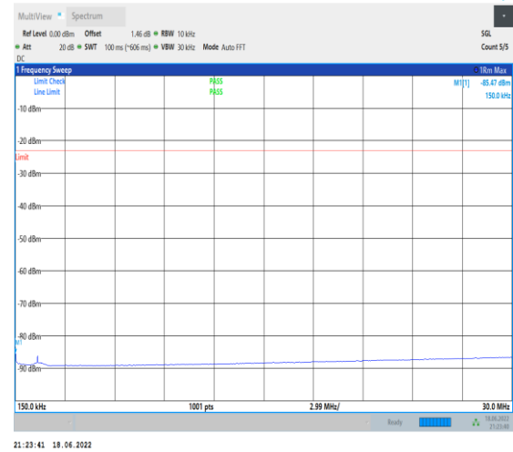
1-N71--15-20-H-1-DFT-PI2BPSK-Inner_1RB_Left-1 @1-0.15-30-Ant1--85.47--23-PASS
