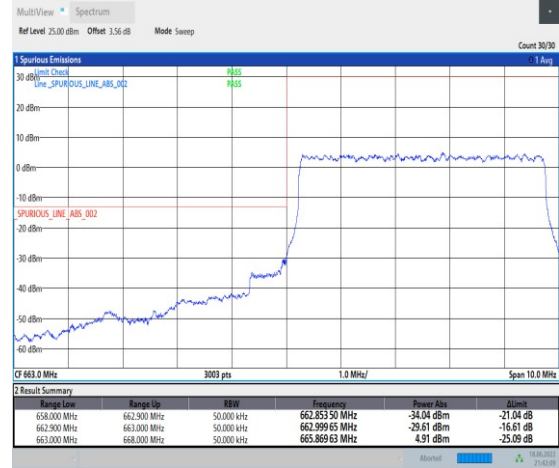
1-N71--15-5-L-3-DFT-PI2BPSK-Outer_Full-25@0-Ant1-PASS-see graph
