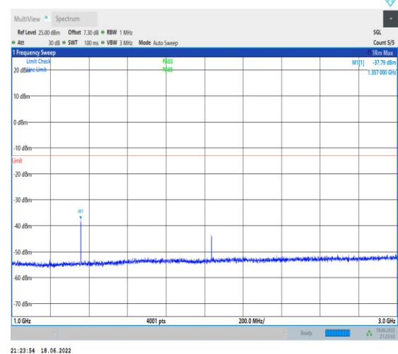
1-N71--15-20-H-1-DFT-PI2BPSK-Inner_1RB_Left-1 @1-1000-3000-Ant1--37.79--13-PASS
