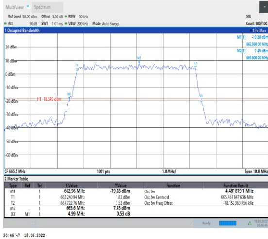
1-N71--15-5-L-9-CP-256QAM-Outer_Full-25@0-Ant1 -4.482-4.990-≤5-PASS
