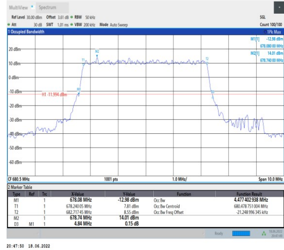
1-N71--15-5-M-1-DFT-QPSK-Outer_Full-25@0-Ant1 -4.477-4.840-≤5-PASS
