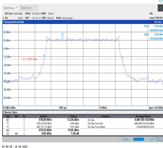
1-N71--15-5-M-2-DFT-PI2BPSK-Outer_Full-25@0-Ant1 -4.465-4.850-≤5-PASS
