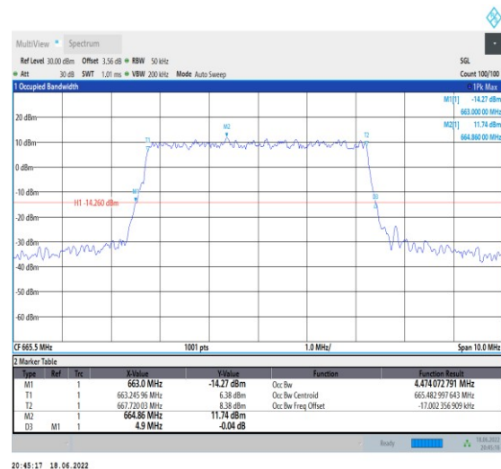
1-N71--15-5-L-4-DFT-64QAM-Outer_Full-25@0-Ant 1-4.474-4.900-≤5-PASS
