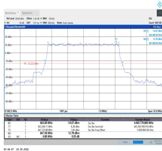
1-N71--15-5-L-2-DFT-P12BPSK-Outer_Full-25@0-An t1-4.466-4.880-≤5-PASS
