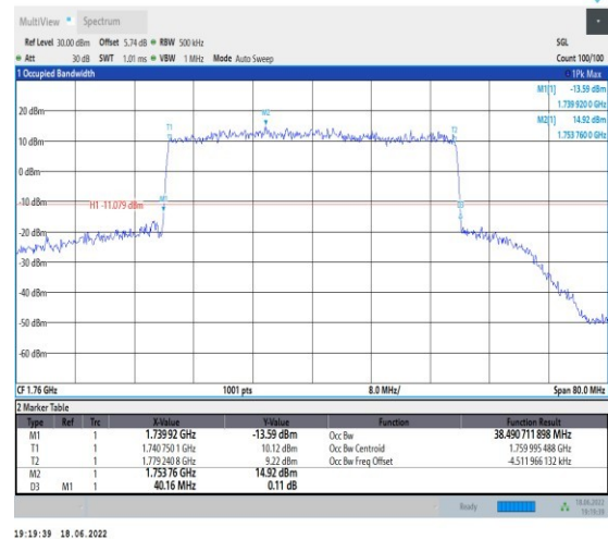
1-N66--15-40-H-3-DFT-16QAM-Outer_Full-216@0-A nt1-38.491-40.160-≤40-PASS
