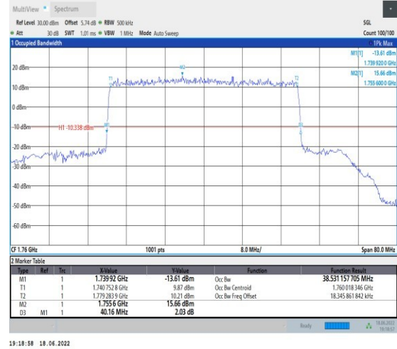
1-N66--15-40-H-1-DFT-QPSK-Outer_Full-216@0-An t1-38.531-40.160-≤40-PASS
