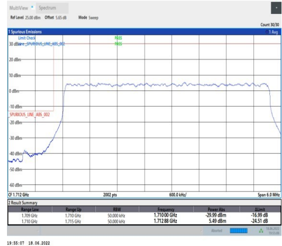
1-N66--15-5-L-3-DFT-PI2BPSK-Outer_Full-25@0-Ant1-seegraph-PASS-see graph
