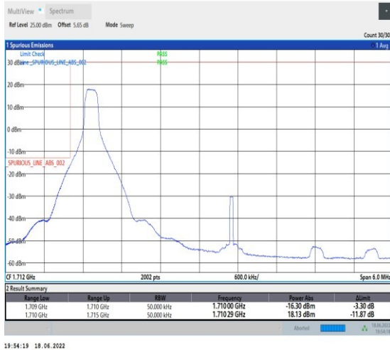
1-N66--15-5-L-1-DFT-PI2BPSK-Edge_1RB_Left-1@0-Ant1-seegraph-PASS-see graph
