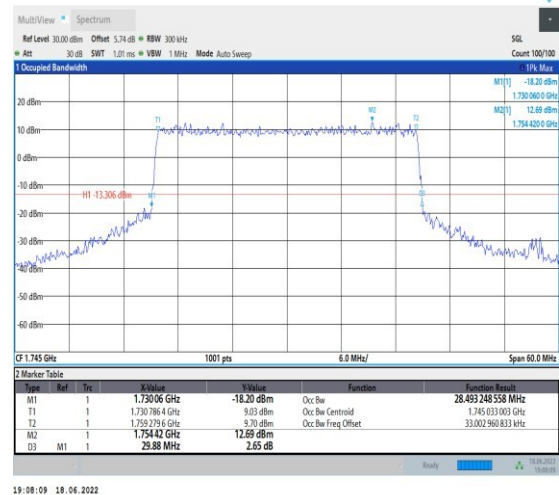
1-N66--15-30-M-7-CP-16QAM-Outet_Full-160@0-A nt1-28.493-29.880-≤30-PASS
