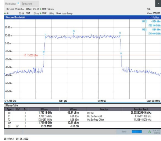
1-N66--15-30-M-5-DFT-256QAM-Outet_Full-160@0-A Ant1-28.553-29.580-≤30-PASS
