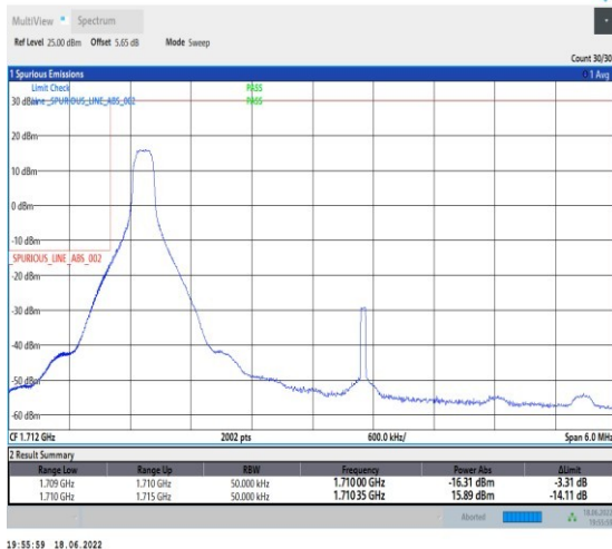
1-N66--15-5-L-4-CP-QPSK-Edge_1RB_Left-1@0-Ant1-seegraph-PASS-see graph
