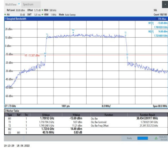
1-N66--15-40-L-3-DFT-16QAM-Outer_Full-216@0-Ant1-38.454-40.160-≤40-PASS
