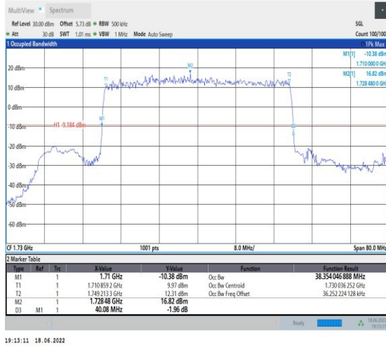
1-N66--15-40-L-2-DFT-PI2BPSK-Outer_Full-216@0-Ant1-38.354-40.080-≤40-PASS
