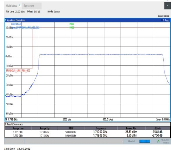
1-N66--15-5-L-6-CP-QPSK-Outer_Full-25@0-Ant1-seegraph-PASS-see graph
