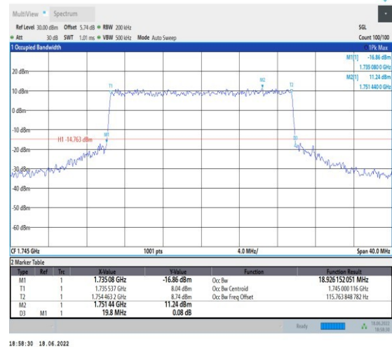
1-N66--15-20-M-6-CP-QPSK-Outer_Full-106@0-Ant 1-18.926-19.800-≤20-PASS
