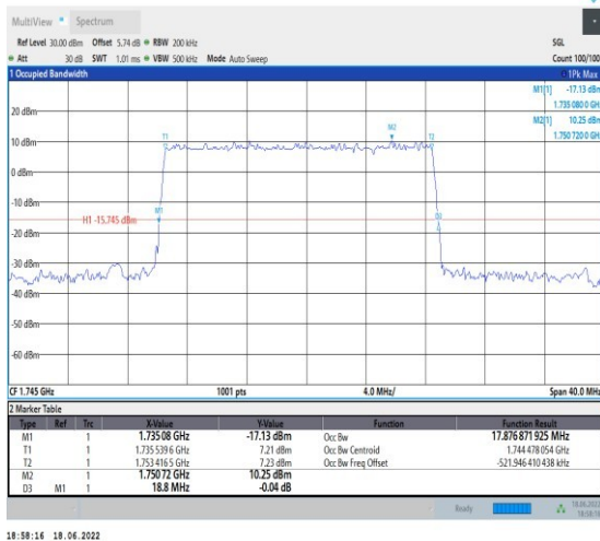
1-N66--15-20-M-5-DFT-256QAM-Outer_Full-100@0-A Ant1-17.877-18.800-≤20-PASS
