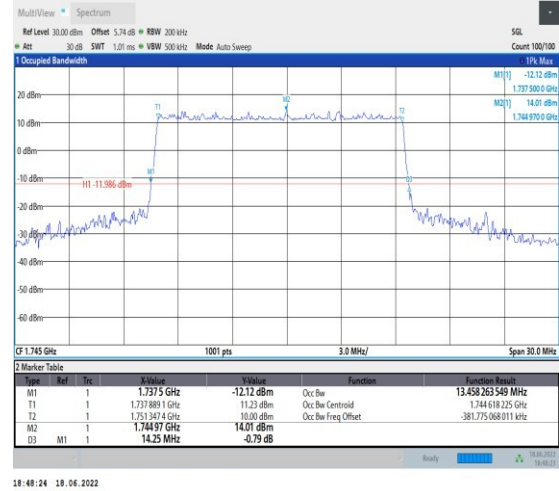
1-N66--15-15-M-3-DFT-16QAM-Outer_Full-75@0-An t1-13.458-14.250-≤15-PASS
