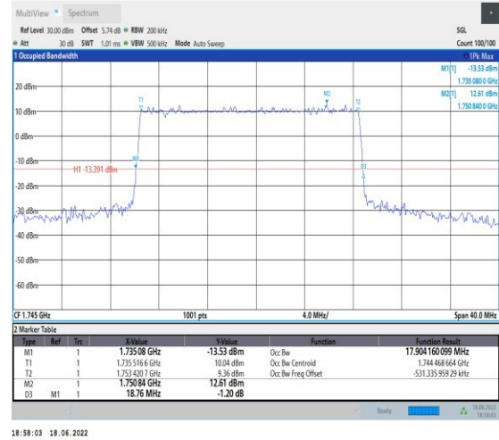
1-N66--15-20-M-4-DFT-64QAM-Outer_Full-100@0-A nt1-17.904-18.760-≤20-PASS
