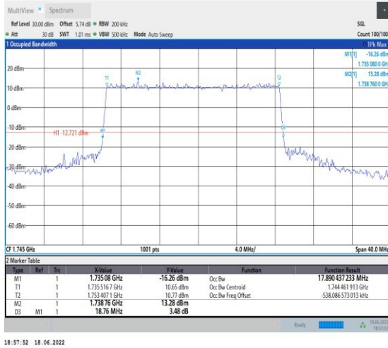
1-N66--15-20-M-3-DFT-16QAM-Outer_Full-100@0-A nt1-17.89-18.760-≤20-PASS
