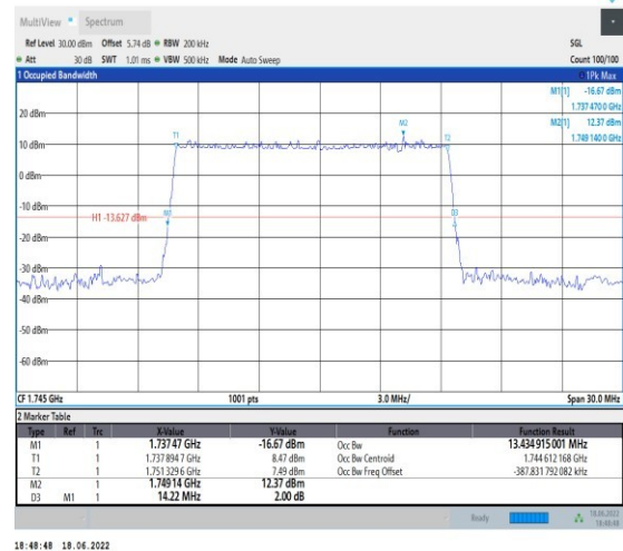
1-N66--15-15-M-5-DFT-256QAM-Outer_Full-75@0-A nt1-13.435-14.220-≤15-PASS
