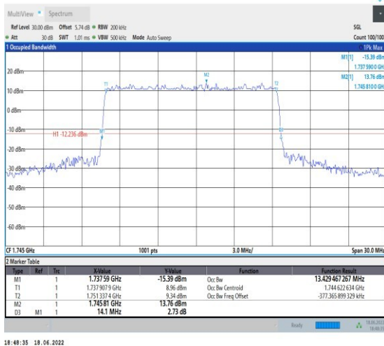
1-N66--15-15-M-4-DFT-64QAM-Outer_Full-75@0-An t1-13.429-14.100-≤15-PASS
