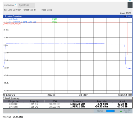
1-N25-PC3-15-25-H-6-CP-QPSK-Outer_Full-133@0-Ant1-seegraph-PASS-see graph
