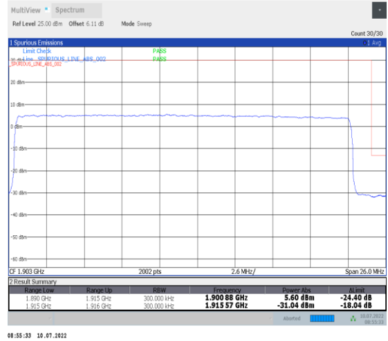
1-N25-PC3-15-25-H-3-DFT-PI2BPSK-Outer_Full-128@0-Ant1-seegraph-PASS-see graph
