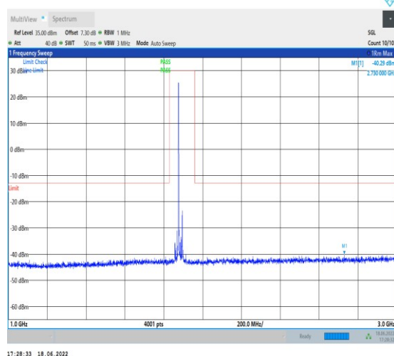
1-N25--15-40-H-1-DFT-PI2BPSK-Inner_1RB_Left-1 @1-1000-3000-Ant1--40.29--13-PASS
