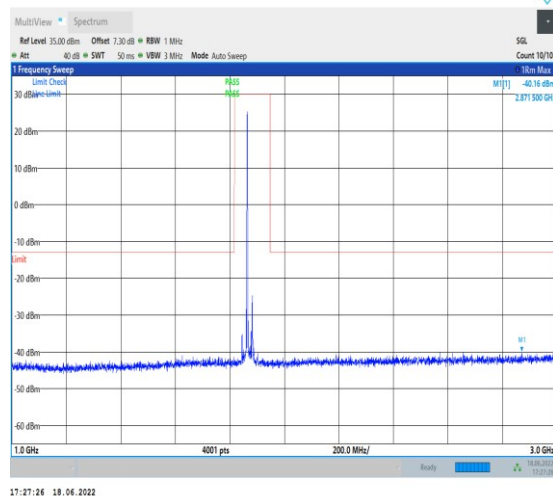
1-N25--15-40-M-1-DFT-PI2BPSK-Inner_1RB_Left-1 @1-1000-3000-Ant1--40.16--13-PASS
