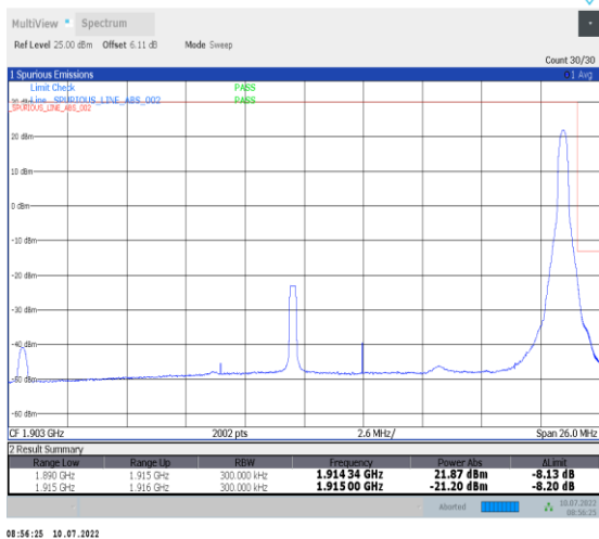
1-N25-PC3-15-25-H-5-CP-QPSK-Edge_1RB_Right-1@132-Ant1-seegraph-PASS-see graph
