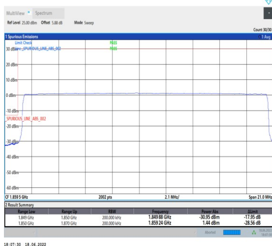
1-N25--15-20-L-6-CP-QPSK-Outer_Full-106@0-Ant1-seegraph-PASS-see graph
