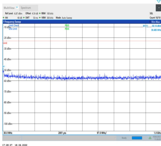
1-N25--15-40-H-1-DFT-PI2BPSK-Inner_1RB_Left-1 @1-30-1000-Ant1--50.14--23-PASS
