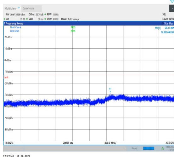
1-N25--15-40-M-1-DFT-PI2BPSK-Inner_1RB_Left-1 @1-12000-20000-Ant1--28.11--13-PASS
