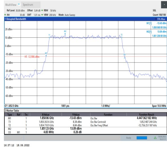
1-N25-PC3-15-5-L-2-DFT-PI2BPSK-Outer_Full-25@ 0-Ant1-4.447-4.830-≤5-PASS
