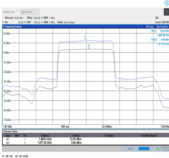
1-N25--15-40-L-1-DFT-256QAM-Outer_Full-216@0-Ant1-9.29-100%-0.00-9.29-PASS-≤13
