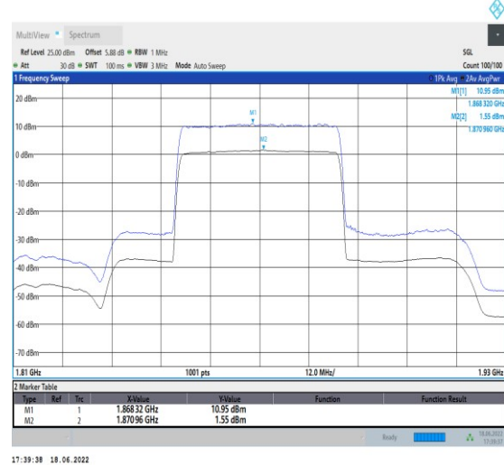
1-N25--15-40-L-2-CP-256QAM-Outer_Full-216@0-Ant1-9.40-100%-0.00-9.40-PASS-≤13
