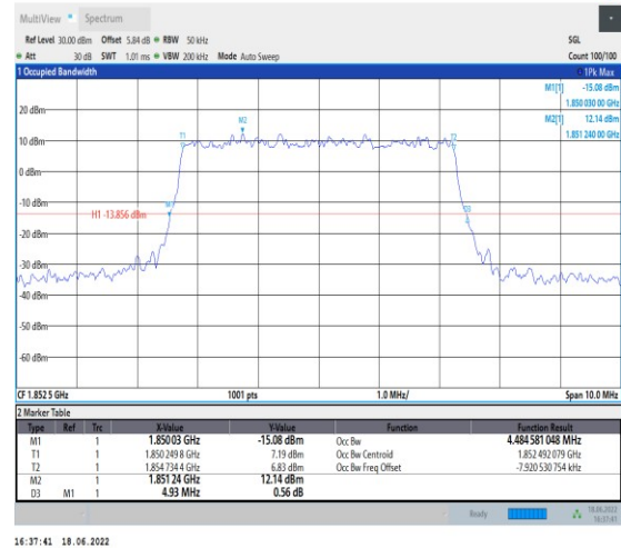
1-N25-PC3-15-5-L-4-DFT-64QAM-Outer_Full-25@0- Ant1-4.485-4.930-≤5-PASS
