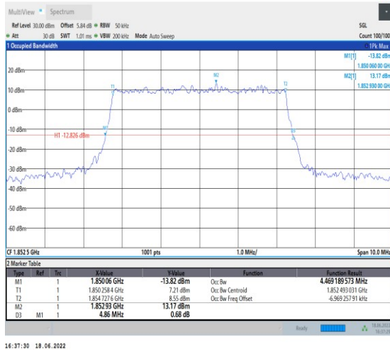
1-N25-PC3-15-5-L-3-DFT-16QAM-Outer_Full-25@0- Ant1-4.469-4.860-≤5-PASS
