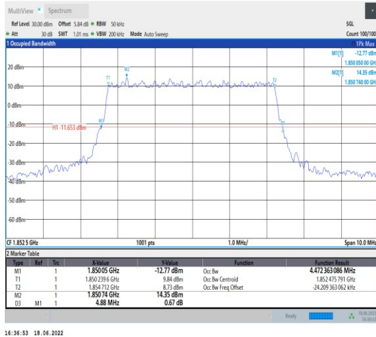
1-N25-PC3-15-5-L-1-DFT-QPSK-Outer_Full-25@0-A nt1-4.472-4.880-≤5-PASS
