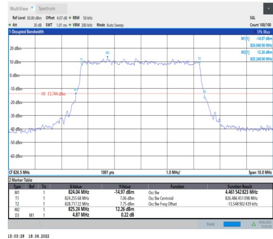
1-N5--15-5-L-4-DFT-64QAM-Outer_Full-25@0-Ant1- 4.462-4.870-≤5-PASS
