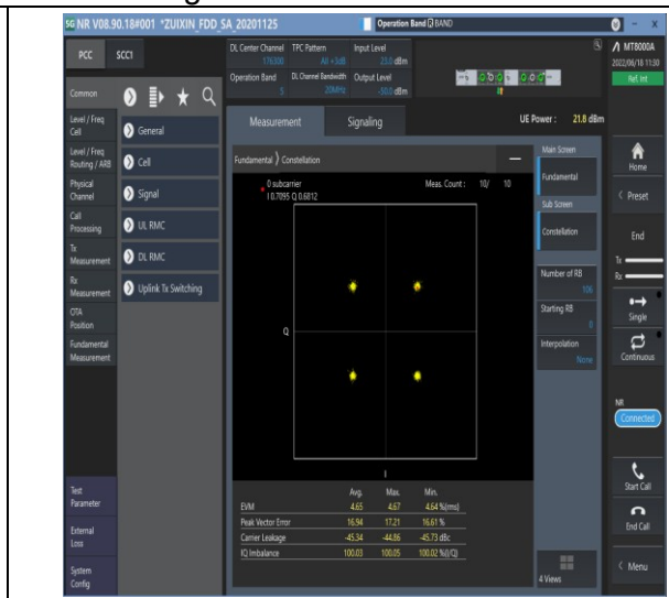
1-N5--15-20-M-6-CP-QPSK-Outer_Full-106@0-Ant 1-see graph-PASS
