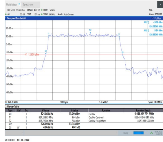
1-N5--15-5-L-2-DFT-PI2BPSK-Outer_Full-25@0-Ant 1-4.466-4.860-≤5-PASS
