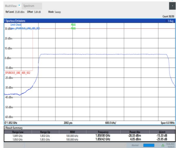
1-N2--15-5-L-6-CP-QPSK-Outer_Full-25@0-Ant1-seegraph-PASS-see graph
