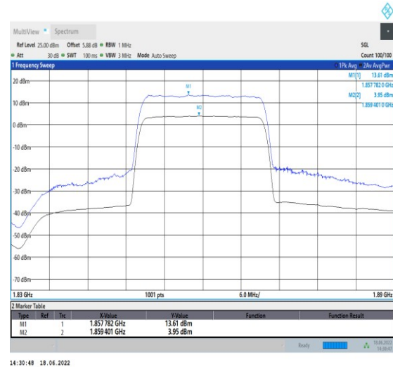
1-N2--15-20-L-2-CP-256QAM-Outer_Full-106@0-An t1-9.66-100%-0.00-9.66-PASS≤13
