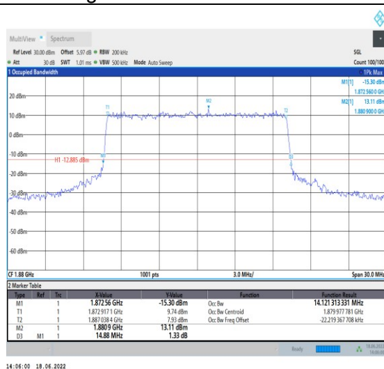
1-N2--15-15-M-7-CP-16QAM-Outer_Full-79@0-Ant1 -14.121-14.880-≤15-PASS
