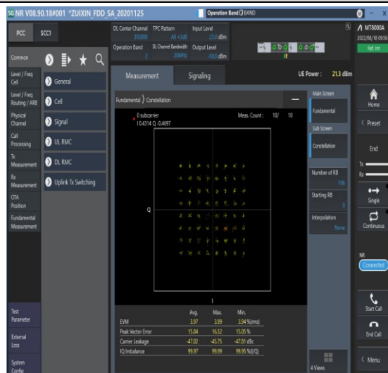
1-N2--15-20-M-8-CP-64QAM-Outer_Full-106@0-Ant1-see graph-PASS
