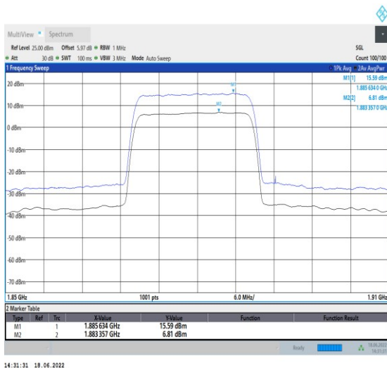
1-N2--15-20-M-1-DFT-256QAM-Outer_Full-100@0-A nt1-8.78-100%-0.00-8.78-PASS≤13
