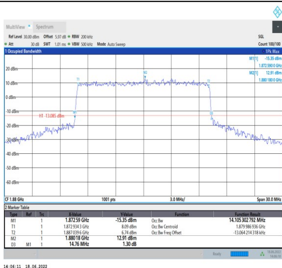
1-N2--15-15-M-8-CP-64QAM-Outer_Full-79@0-Ant1 -14.105-14.760-≤15-PASS
