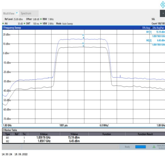
1-N2--15-20-L-1-DFT-256QAM-Outer_Full-100@0-A nt1-8.74-100%-0.00-8.74-PASS≤13
