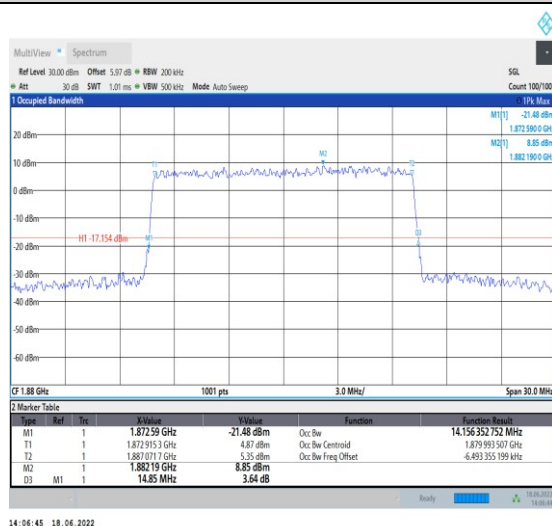
1-N2--15-15-M-9-CP-256QAM-Outer_Full-79@0-Ant 1-14.156-14.850≤15-PASS
