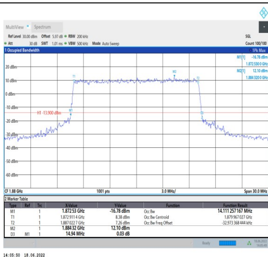
1-N2--15-15-M-6-CP-QPSK-Outer_Full-79@0-Ant1- 14.111-14.940-≤15-PASS
