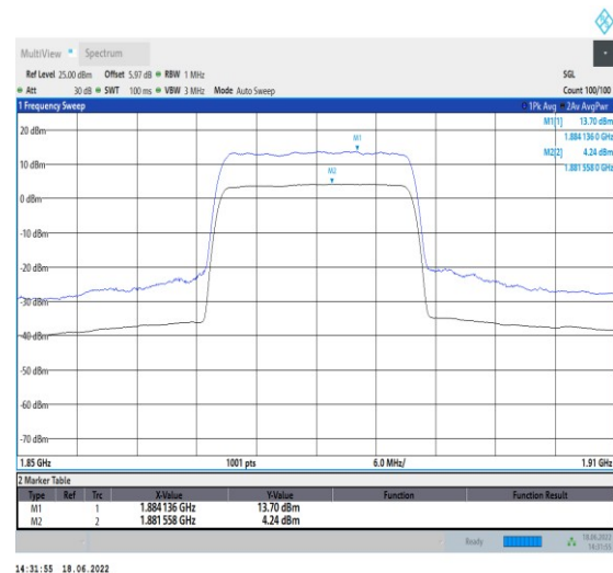
1-N2--15-20-M-2-CP-256QAM-Outer_Full-106@0-A nt1-9.46-100%-0.00-9.46-PASS≤13
