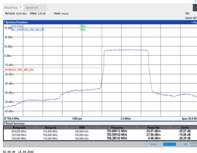
Band17-5MHz-QPSK-23755-25RB#0
