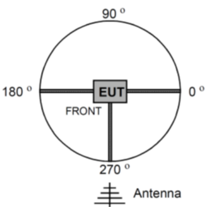
Picture 4.4.1 Turntable azimuth variations.
