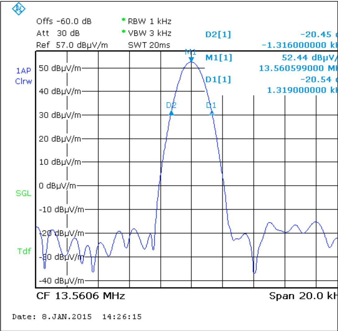
Figure 4.5.2.1 20 dB Bandwidth of the modulated carrier.
