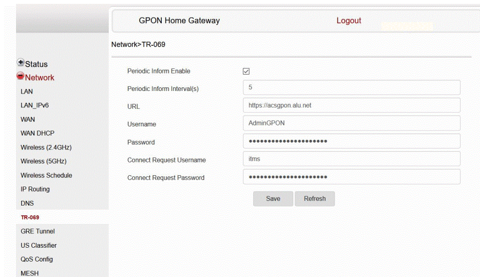
Figure 7-24 TR-069 page
