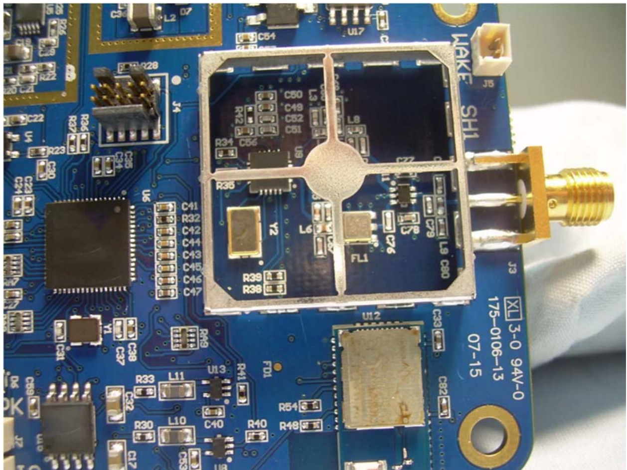
View of the RF Circuitry of the 902 – 928 MHz Transmitter and Receiver
