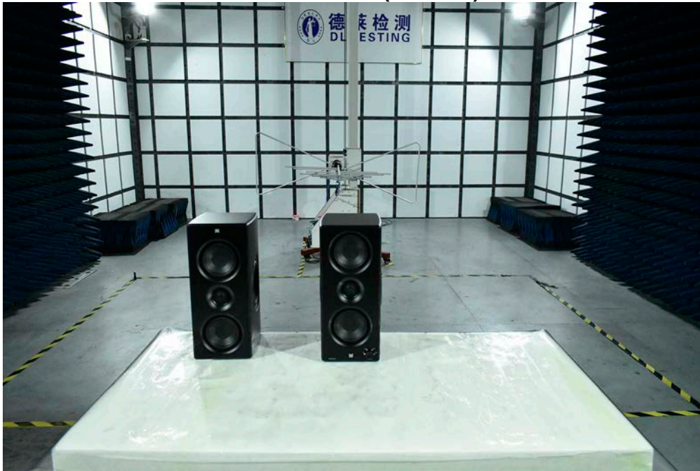
RadiatedEmission(Below 1G)
