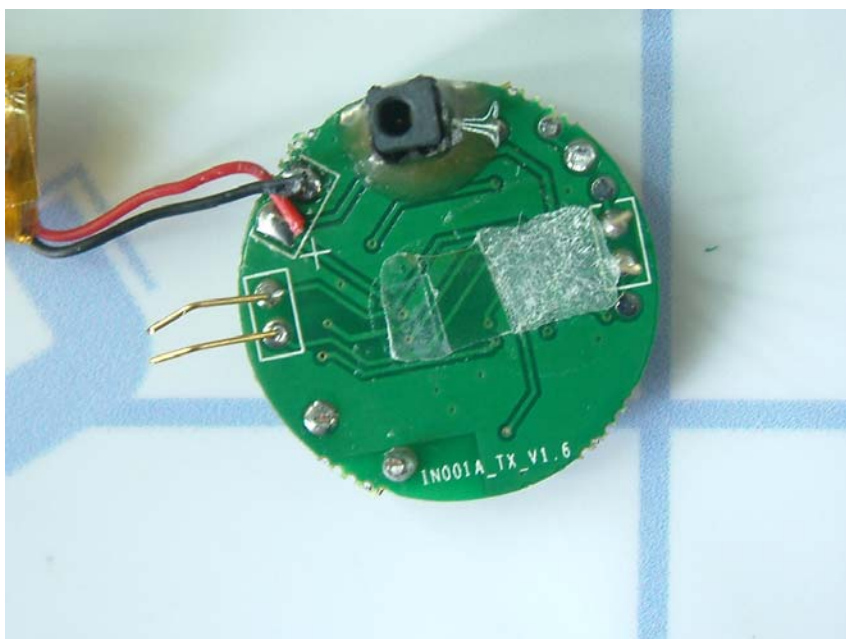
TX PCB side 2
