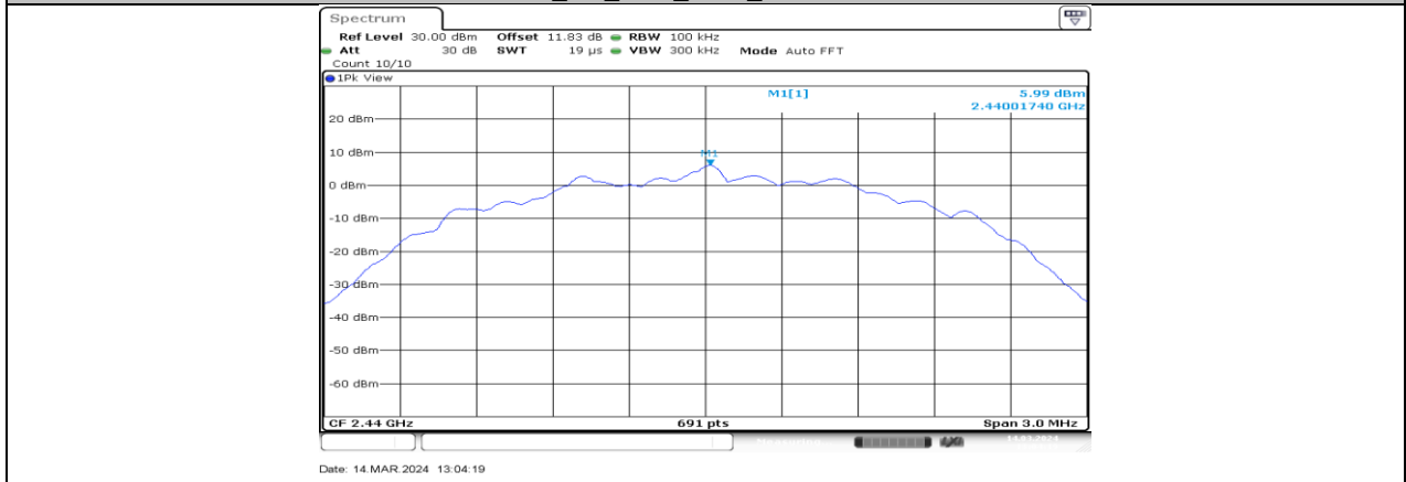
BLE_2M_Ant2_2440_0~Reference
