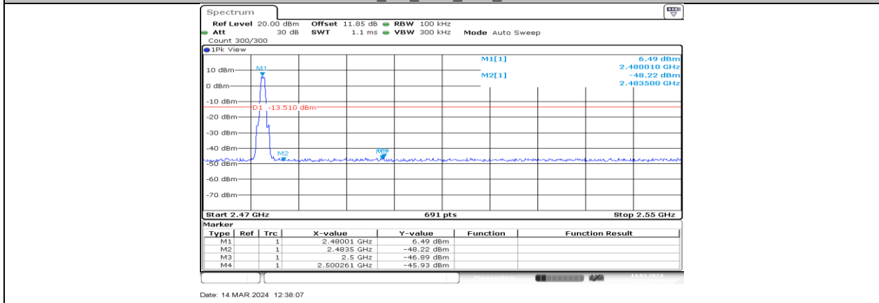
BLE_1M_Ant2_High_2480
