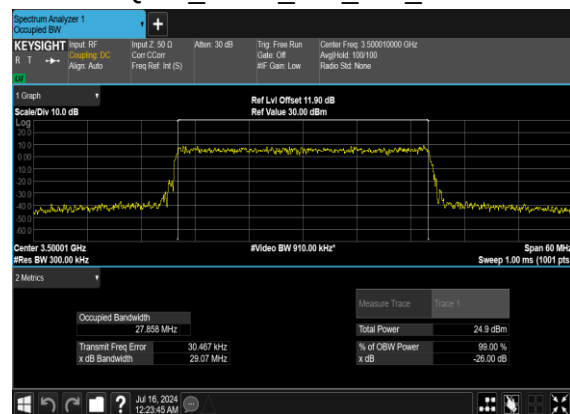
N77(30M)_CP-OFDM_256 QAM_Outer_Full_Mid_CH
