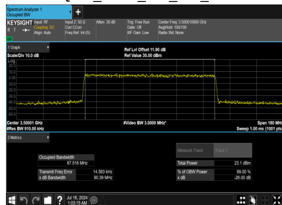
N77(90M)_CP-OFDM_256 QAM_Outer_Full_Mid_CH
