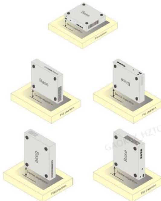
Picture D.5 Test positions for desktop devices
