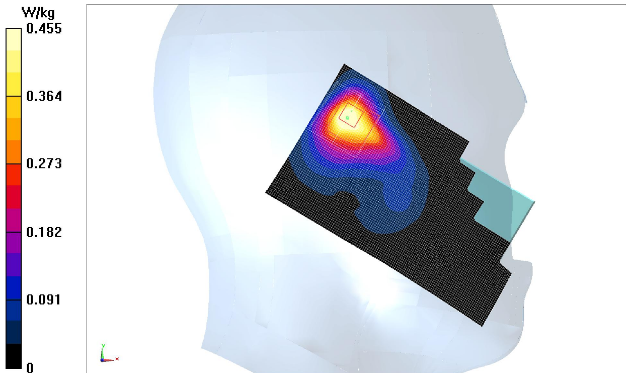
Fig.9 2450 MHz CH6
