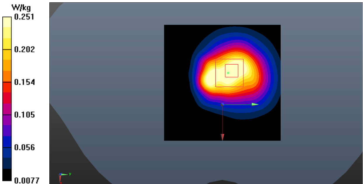
Fig.16 LTE Band 5
