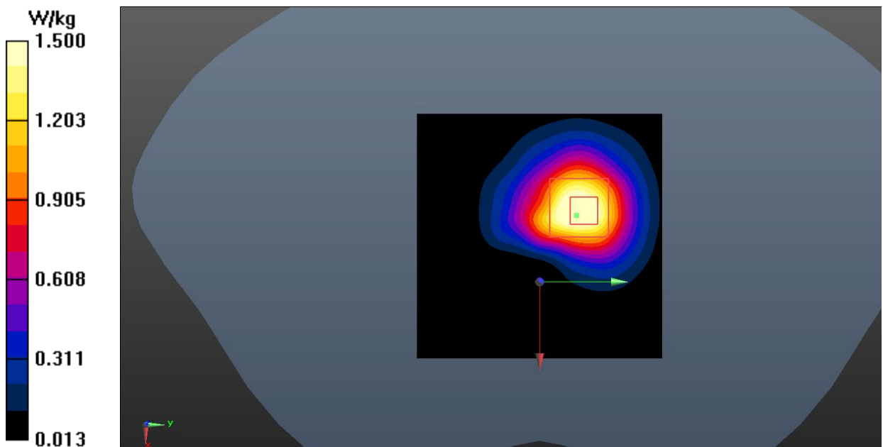
Fig.10 WCDMA 1700
