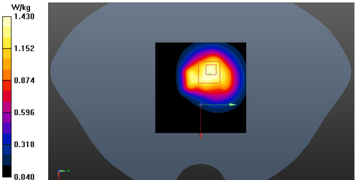
Fig.2 GSM 850 MHz
