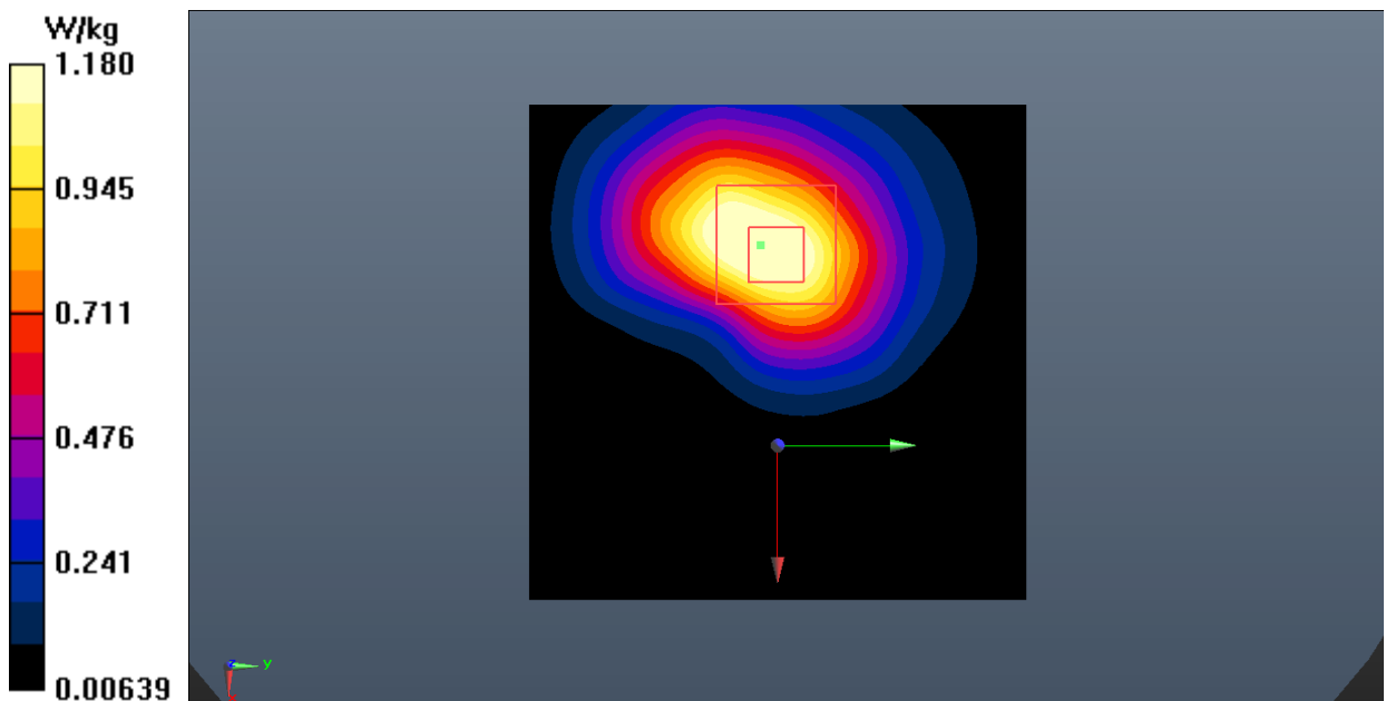
Fig.7 WCDMA 1900
