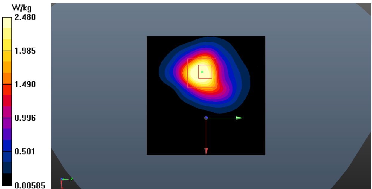
Fig.18 LTE Band 7
