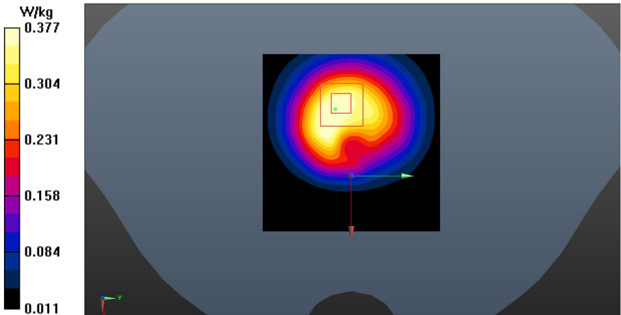
Fig.1 GSM 850 MHz
