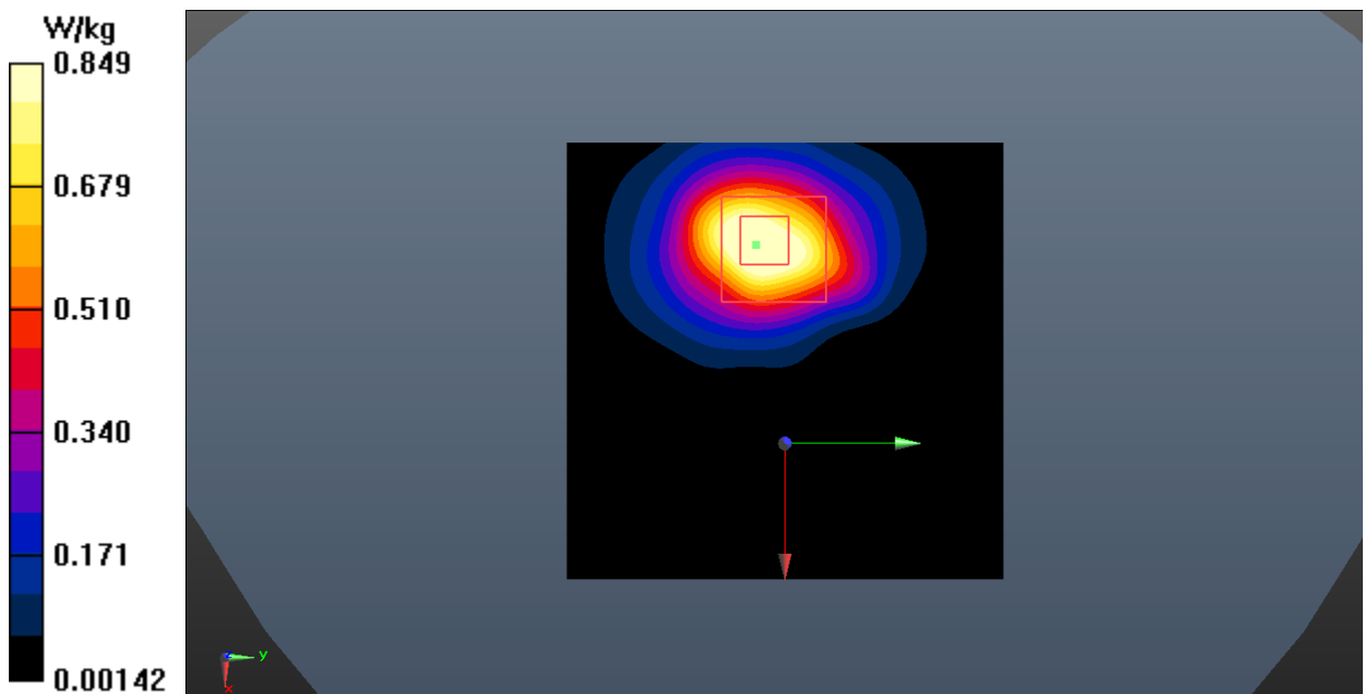
Fig.20 WLAN 2.4G
