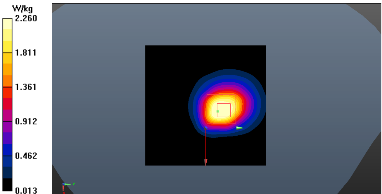
Fig.8 WCDMA 1900
