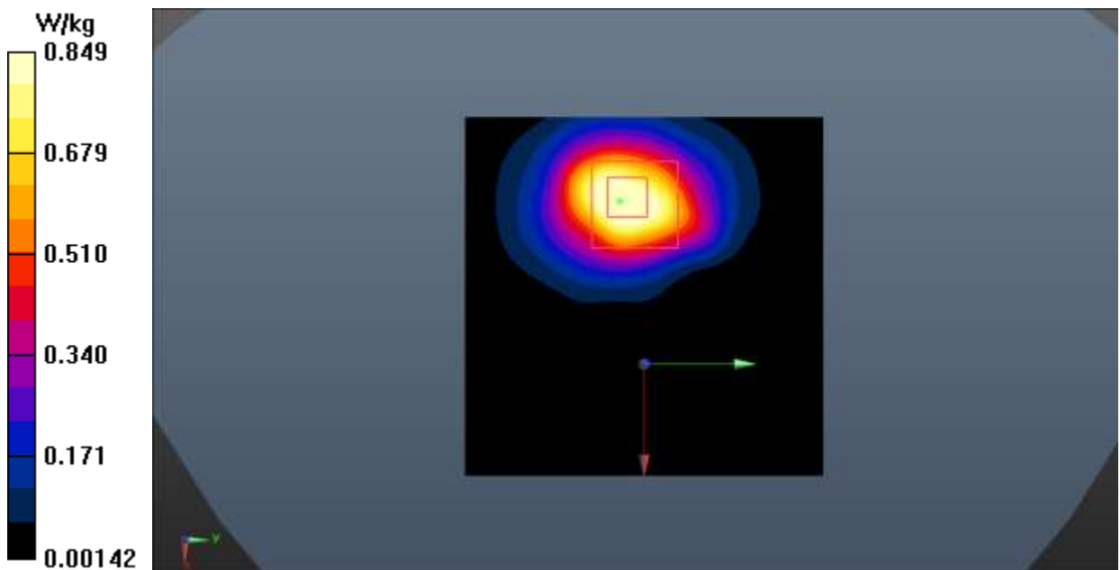
Fig.20 Wi-Fi 2.4G
