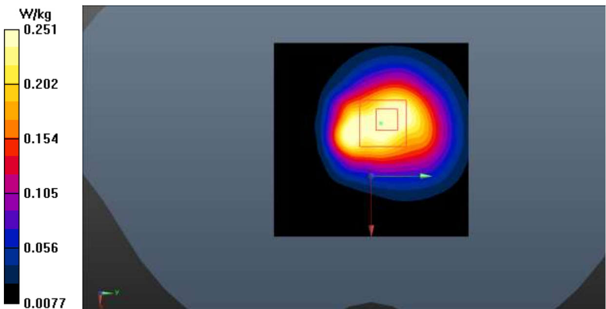
Fig.16 LTE Band 5
