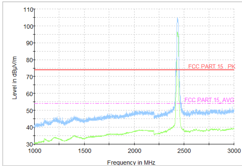
Fig.52 Radiated Spurious Emission (802.11n HT20, CH6, 1 GHz-3 GHz)
