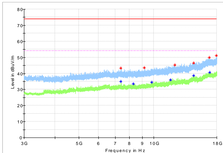
Fig.55 Radiated Spurious Emission (802.11n HT20, CH11, 3 GHz-18 GHz)
