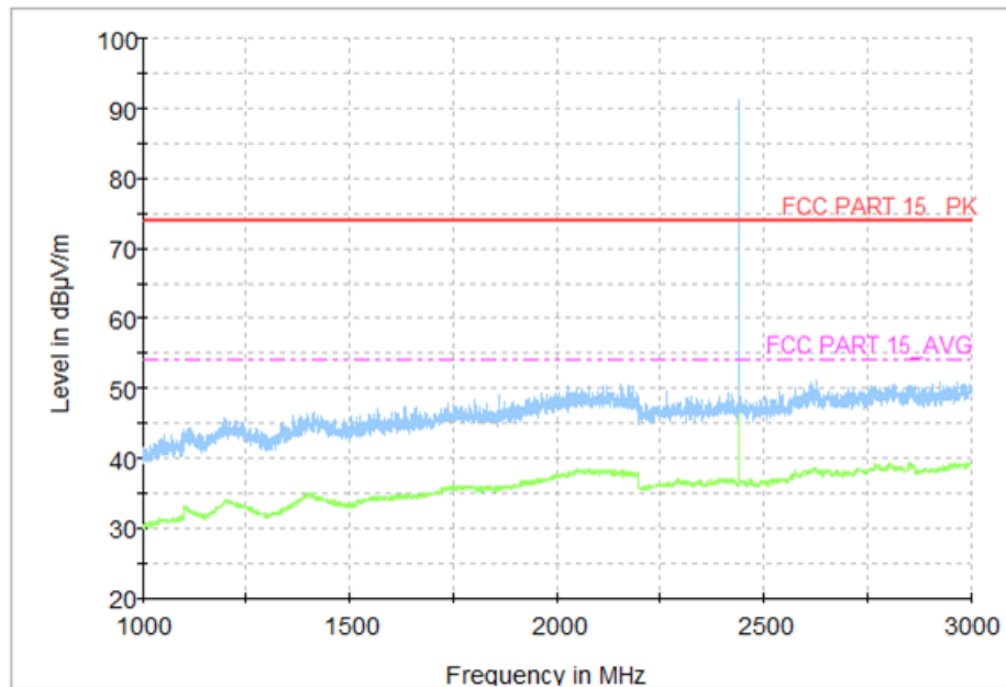
Fig.22 Radiated Spurious Emission (GFSK, Ch19, 1 GHz ~3 GHz)
