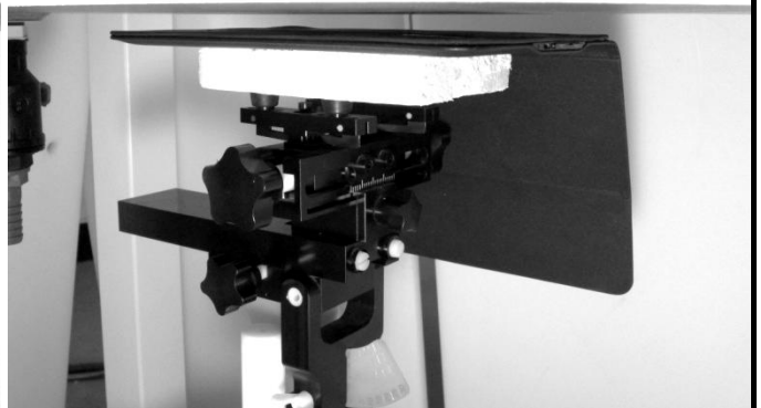
Front Face of EUT with 1.1 cm Gap
