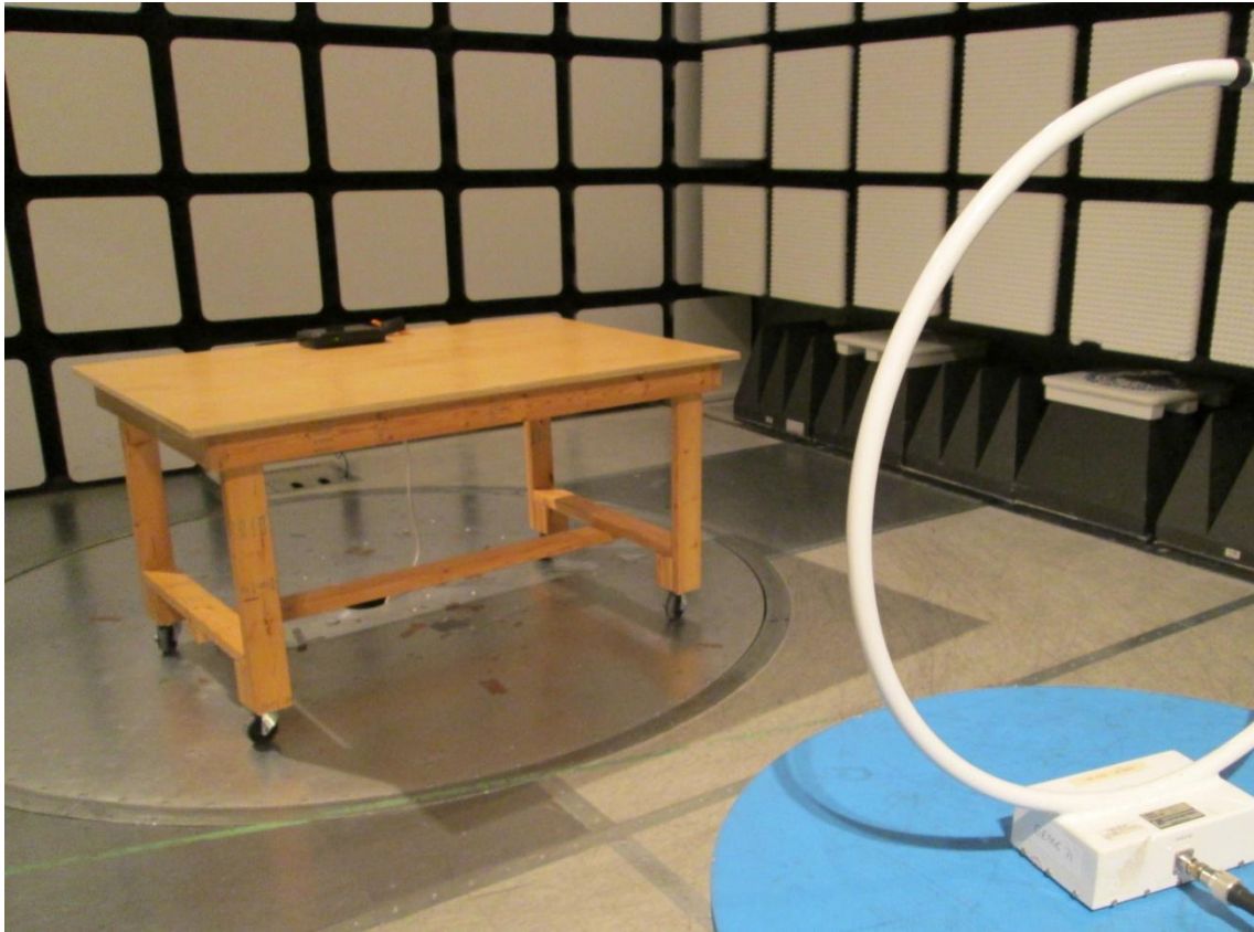
Photo 3. Radiated Emissions 3
