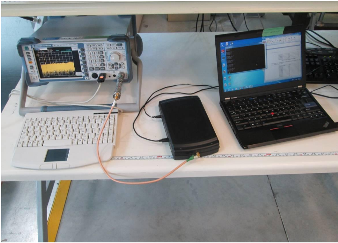
Photo 4. Conducted Measurements
