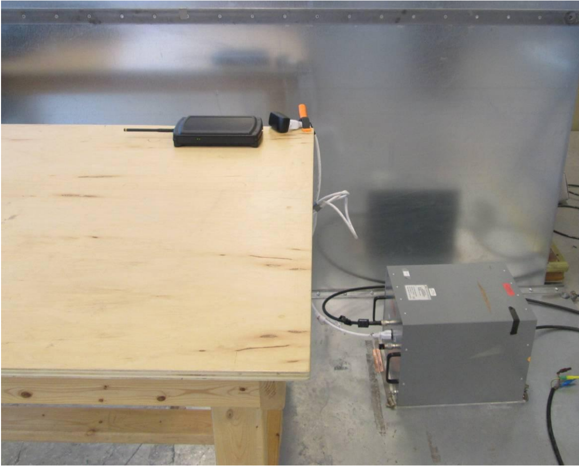
Photo 5. Power Line Conducted Emissions
