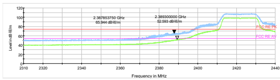
802.11n HT20 -Channel 3 Peak+ Average
