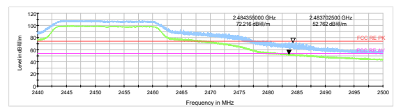
802.11n HT20 -Channel 9 Peak+ Average
