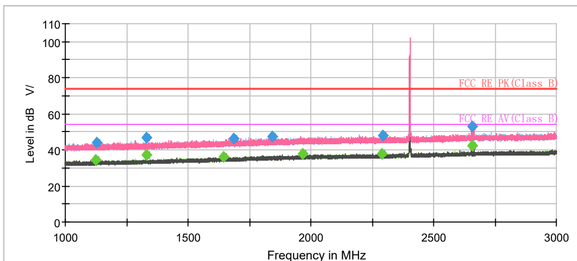
Radiates Emission from 1GHz to 3GHz
