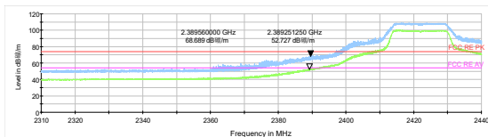
802.11g-Channel 3 Peak+ Average
