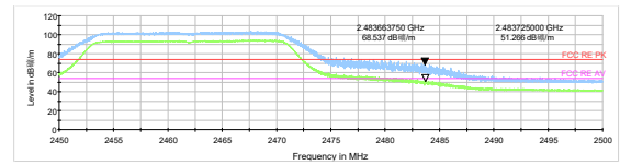
802.11n HT20 -Channel 11 Peak+ Average
