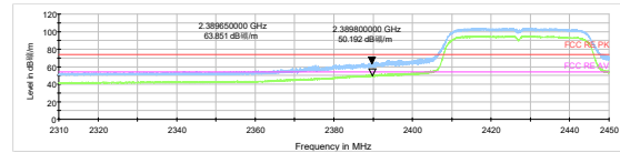
802.11n HT40 –Channel 4 Peak+ Average
