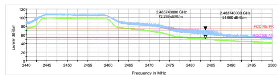
802.11g-Channel 9 Peak+ Average
