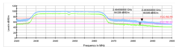
802.11n HT40 –Channel 8 Peak+ Average
