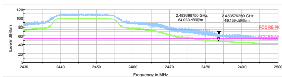
802.11g-Channel 8 Peak+ Average
