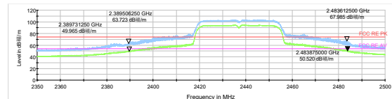
802.11n HT40 –Channel 6 Peak+ Average
