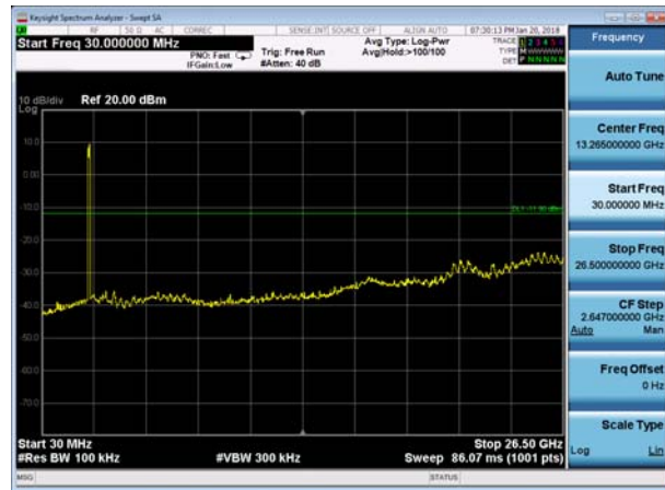
GFSK-CH78 30MHz to 26.5GHz
