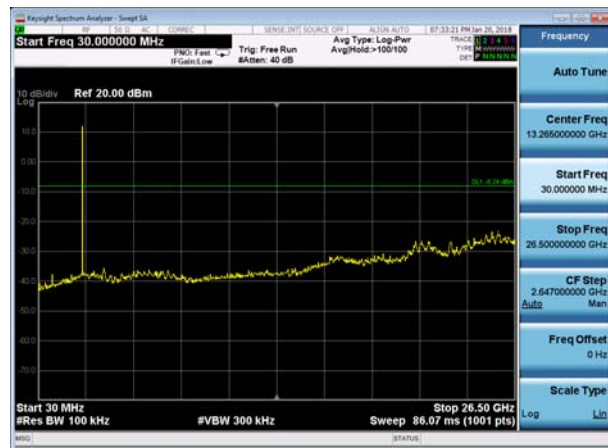
DQPSK-CH39 30MHz to 26.5GHz
