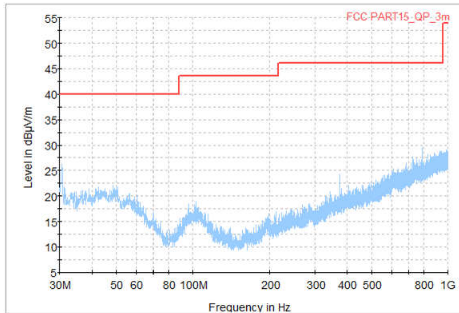
Fig. 67 Radiated Spurious Emission (All Channels, 30 MHz ~1 GHz)
