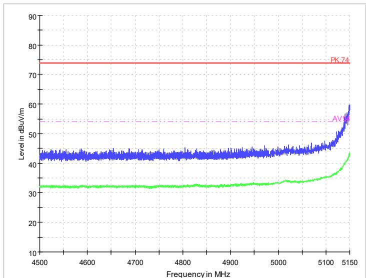
Radiated Emission Band Edge Channel No.:36 Test Mode: 802.11ac Polarization: H
