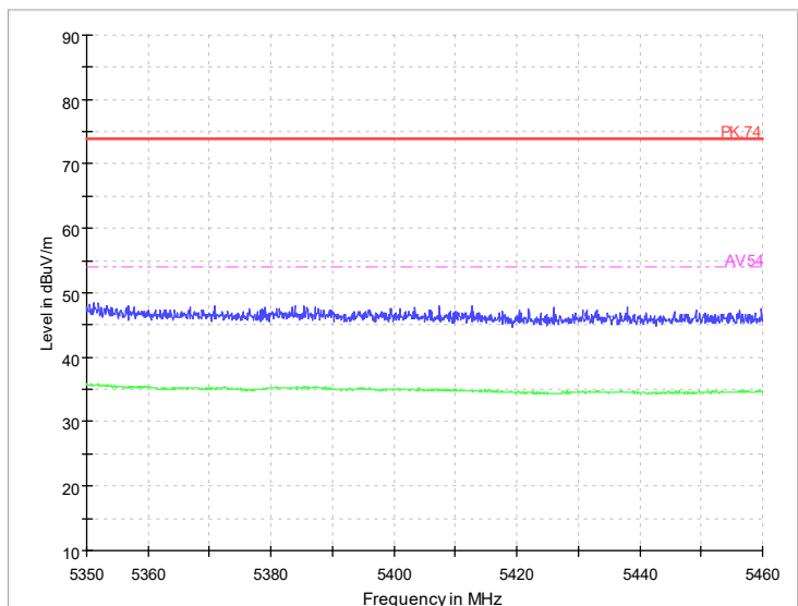
Radiated Emission Band Edge Channel No.:46 Test Mode: 802.11n Polarization: V
