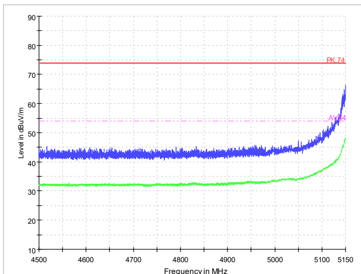
Radiated Emission Band Edge Channel No.:38 Test Mode: 802.11ac Polarization: H
