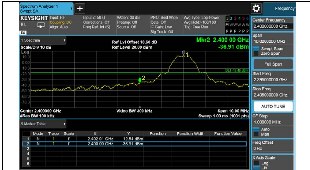
BLE-2402MHz
