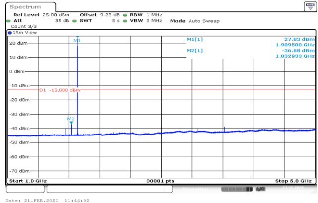
GPRS_1900_Higher(1GHz-5GHz)
