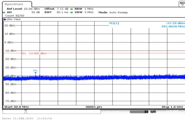
GPRS_1900_Higher(30MHz-1GHz)
