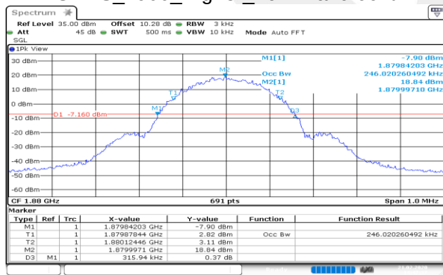
EGPRS(8PSK)_1900_Middle_26BW and 99%
