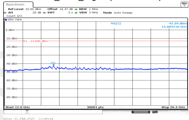
GPRS_1900_Higher(12GHz-26.5GHz)
