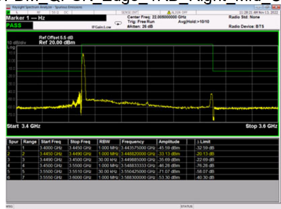
n77(100M)_DFT-s-OFDM QPSK Edge_1RB_Right_Mid_CH
