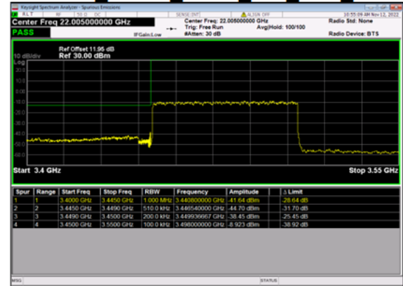
n77(60M)_DFT-s-OFDM QPSK Outer Full Low CH
