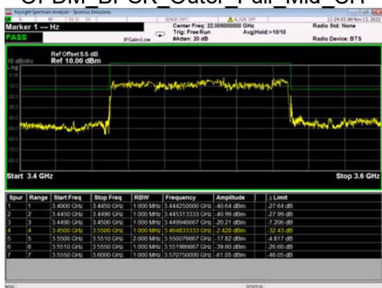
n77(100M)_DFT-s-OFDM BPSK Outer_Full_Mid_CH
