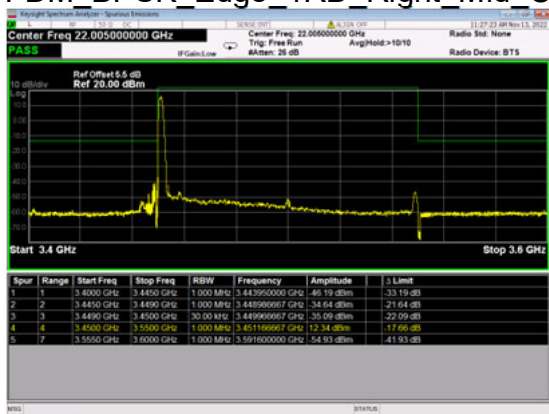
n77(100M)_DFT-s-OFDM BPSK Edge_1RB_Right_Mid_CH
