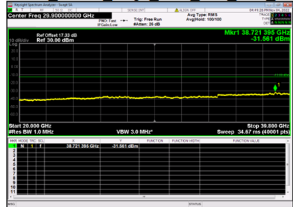
n77(30M)_DFT-s-OFDM QPSK Edge 1RB Left Low CH
