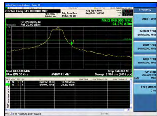
Band26 / 3MHz / High CH / QPSK / 1 RB
