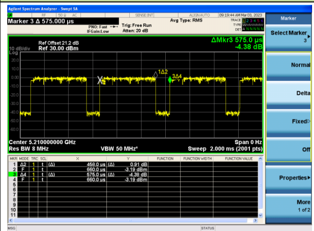
802.11ac-VHT80 (T = 458.0us)
