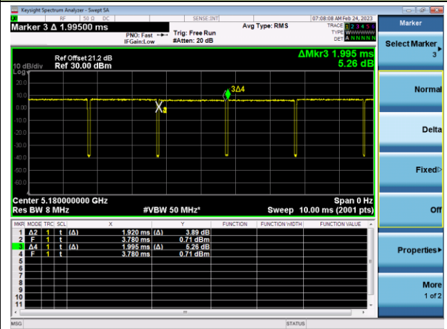
802.11ac-VHT20 (T = 980.0us)
