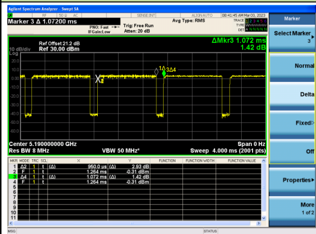
802.11ac-VHT40 (T = 950.0us)
