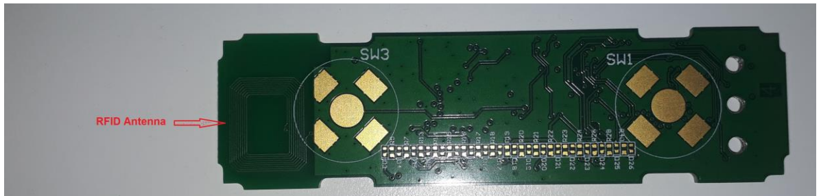
HMI without components, bottom view of PCB
